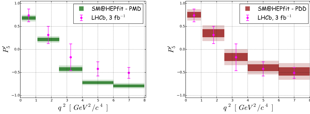
Figure 1: The posterior of P_5' in the PMD (left panel) and PDD (right panel) fits compared with the LHCb measurements.
