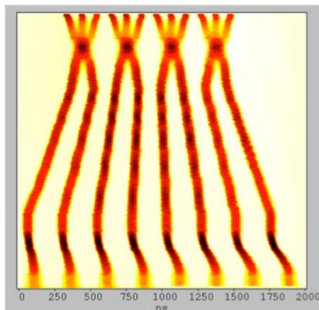
Figure 4: RF gymnastics performed in the PS in order to generate the BCMS beam.
