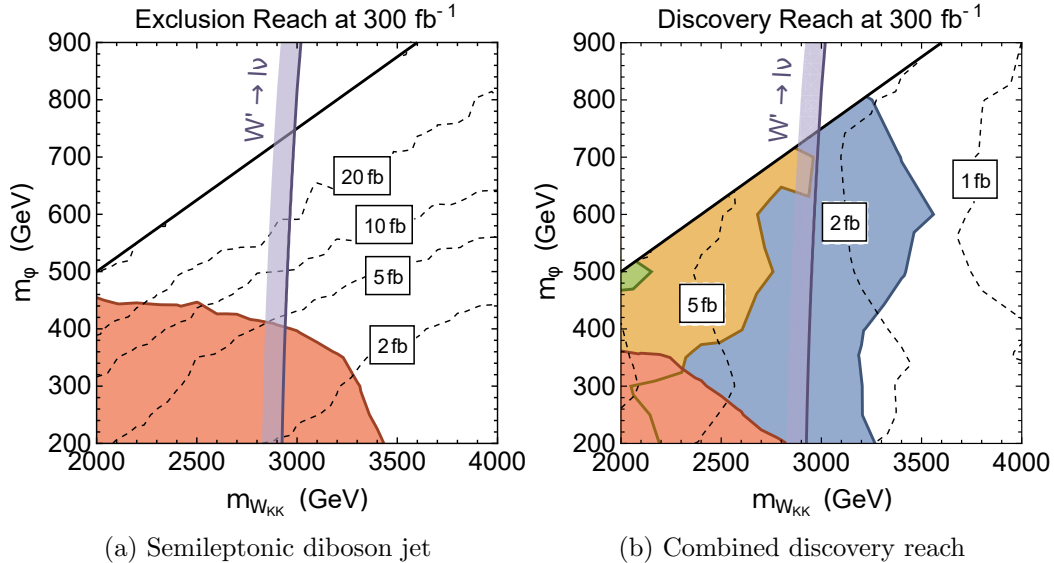
Figure 12: Left: Exclusion reach with \mathcal{L} = 300 \text{ fb}^{-1} for a semi-leptonic diboson jet recoiling against a hadronic W jet. Right: Combined discovery reach with \mathcal{L} = 300 \text{ fb}^{-1} . Red: qq(\ell\nu qq) , orange: \ell\nu(qqqq) , green: qq(qqqq) , blue: combination. Dashed contours indicate the exclusion or combined discovery cross section for W_{KK} \rightarrow W\varphi \rightarrow W(WW) . The purple line indicates the current exclusion due to the search for W' \rightarrow \ell\nu of Ref. [33].
