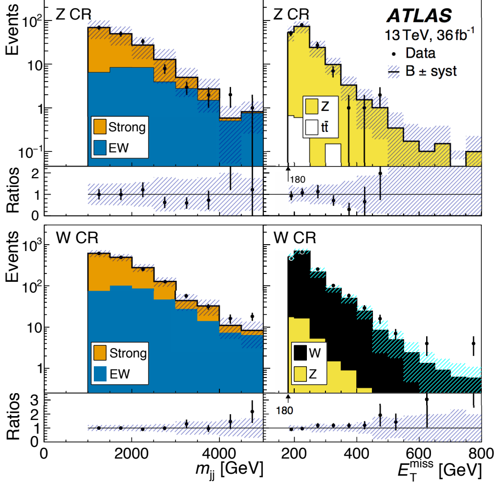
Figure 2: Distribution of event yields in the Z (top) and W (bottom) control regions. The postfit normalizations for m_{jj} (left) and E_T^{\text{miss}} (right) are summed over the subsamples. The E_T^{\text{miss}} distributions start at 180 GeV as indicated. The observed data N (dots) are superimposed on the sum of the backgrounds B (stacked histogram with shaded systematic uncertainty bands). The breakdown of the B is given in the lower left box in each panel. The bottom panels show the ratios of N to B with the systematic uncertainty band shown on the line at 1. The “other,” as listed in Table 1, contribute a few events at low values of m_{jj} and E_T^{\text{miss}} , and are omitted. The last bin in each plot contains the overflow.
