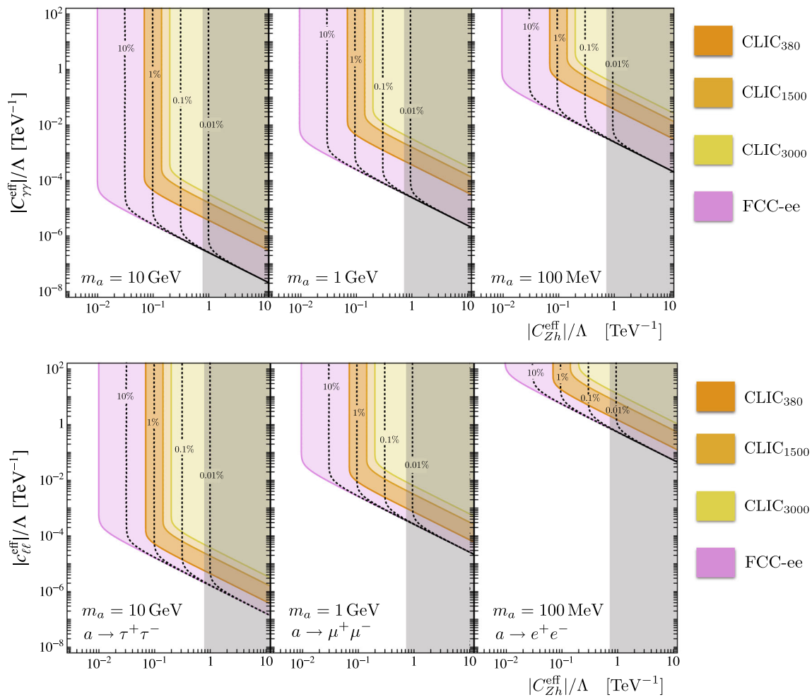
Fig. 8 Parameter regions which can be probed for e^+e^- \rightarrow ha \rightarrow b\bar{b}\gamma\gamma (upper panels) and e^+e^- \rightarrow ha \rightarrow b\bar{b}l^+l^- (lower panels) at future e^+e^- colliders. The grey shaded area is excluded by LHC Higgs measurements. The parameter space to the right of the dotted contours
