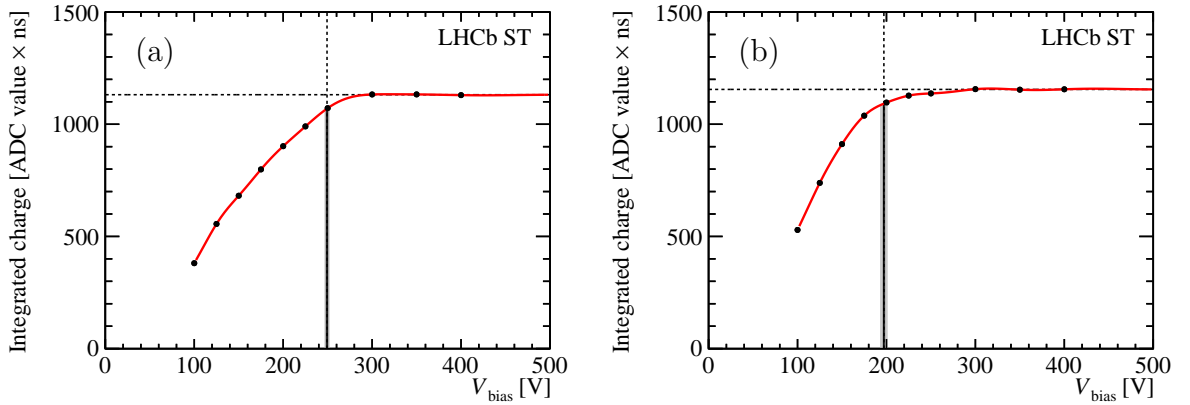
Figure 7: Integrated charge as a function of the applied bias voltage for a central TT read-out sector measured in the CCE scans from (a) April 2012 and (b) September 2017. The decrease of V_{\text{depl}} is clearly visible.
