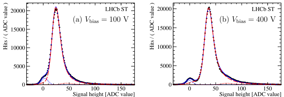
Figure 5: Signal height distribution for hits associated to tracks in the TT for two different bias voltage values. The fitted distribution is described in the text.
