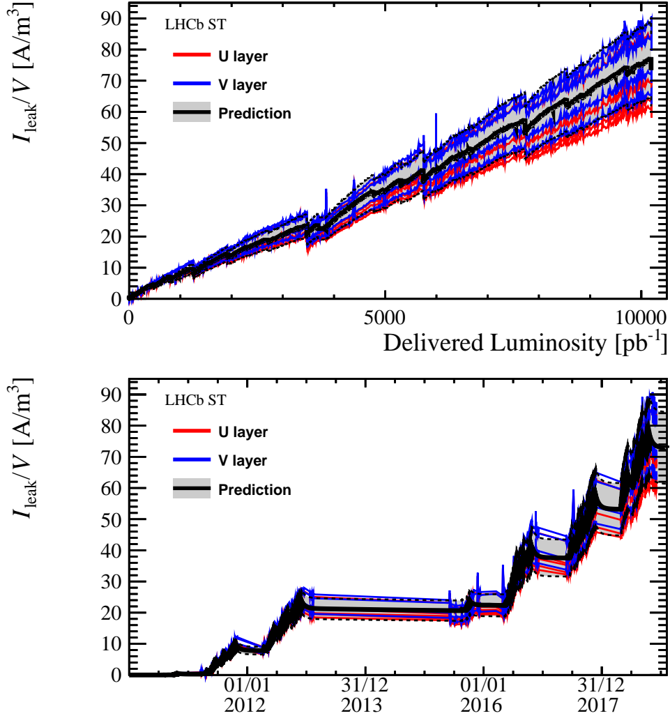
Figure 4: Evolution of the leakage current for the different HV channels connected to one-sensor read-out sectors in TT as a function of (a) the delivered integrated luminosity measured and (b) time. The red curves show channels in the detector layer TTaU, the blue one in TTbV. The predicted evolution is shown in black while the grey band shows its uncertainty, computed from the uncertainty on the model parameters, on the FLUKA simulation and on the temperature measurements. The uncertainty does not account for the range of fluence expected across the sectors shown.
