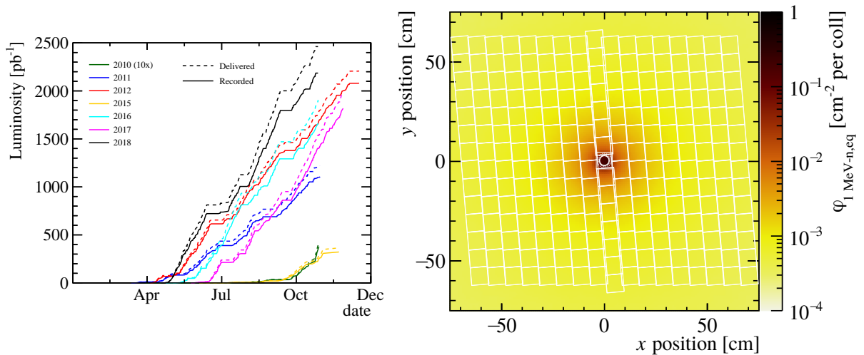
Figure 3: Left: evolution of the integrated luminosity for pp collisions in each year of LHC operation. Right: expected 1- MeV neutron equivalent fluence per proton-proton collision, with the TTaU detector layer overlaid. These results were obtained from a FLUKA simulation of the LHCb detector, assuming a proton-proton collision energy of 14 TeV.
