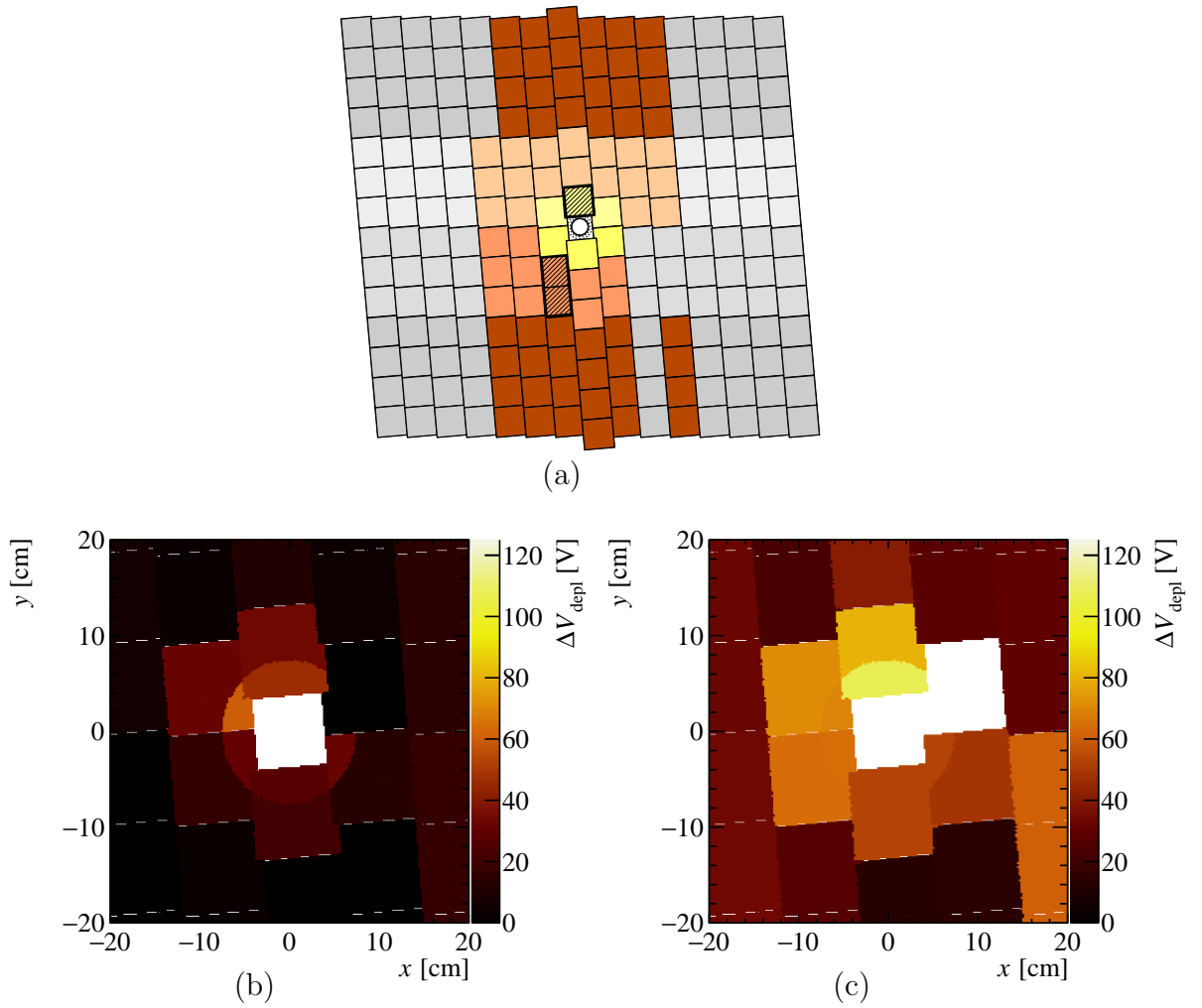
Figure 11: Sketch highlighting the TT sectors analysed during the various CCE scans (a). The greyed out sectors were excluded due to poor statistics. The two sectors highlighted with dashes, just above the beam pipe and below the beam pipe on the left hand side, are those which evolution is shown in Figure 9(a) and Figure 9(b), respectively. Absolute change in V_{\text{depl}} in the innermost region of TT in January 2013 and September 2018 is shown in (b) and (c) respectively. The white sector in (c) became inoperative in August 2017 due to an HV connector issue.
