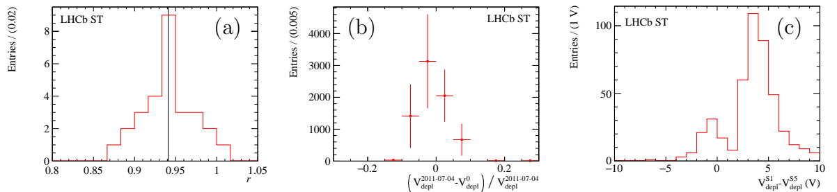
Figure 8: Distributions for all analysed read-out sectors of (a) the ratio r defined in Eq.7; (b) the relative difference between V_{\text{depl}} and V_{\text{depl}}^{2011-07-04} as discussed in the main text; (c) the differences in V_{\text{depl}} obtained from a fifth-order spline and from a linear interpolation. The solid black line in (a) highlights the value of the average \bar{r} .
