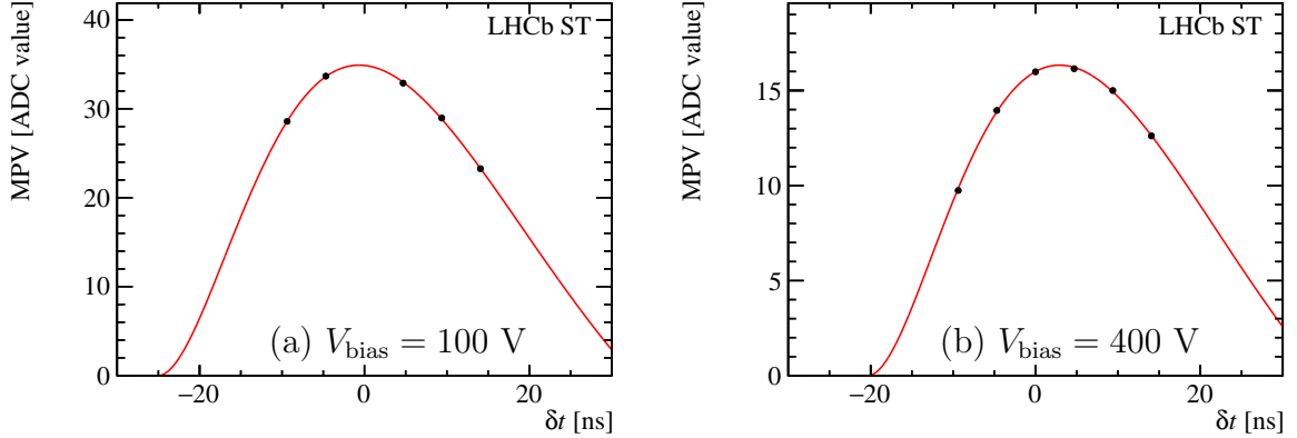
Figure 6: Pulse shapes recorded in the TT for two different bias voltage values. The fitted function is shown in Eq. (6).
