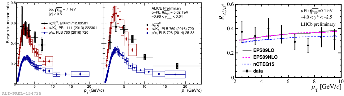
Figure 10: Measurements of \Lambda_c^+ production in small systems at the LHC. Left: \Lambda_c^+/D^0 production ratio in pp and p–Pb collisions in ALICE, compared with light-flavour particles. Right: \Lambda_c^+/D^0 production ratio in LHCb, compared with theoretical model calculations.
