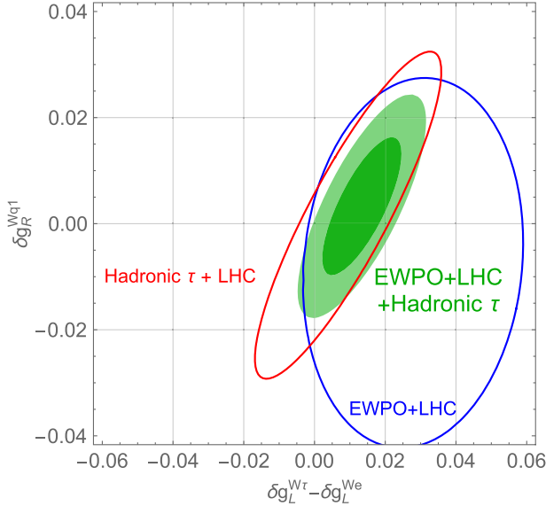
FIG. 1. 68% and 95% C.L. bounds on the vertex corrections \delta g_L^{W\tau} - \delta g_L^{We} and \delta g_R^{Wq1} (green) after using the LHC input to constrain [c_{\ell q}^{(3)}]_{\tau\tau 11} and [c_{\ell q}^{(3)}]_{ee 11} . We also show separate 95% C.L. contours from hadronic \tau decays (red) and from previous EWPO [68] (blue), which are correlated, cf. discussion below Eq. (5).
