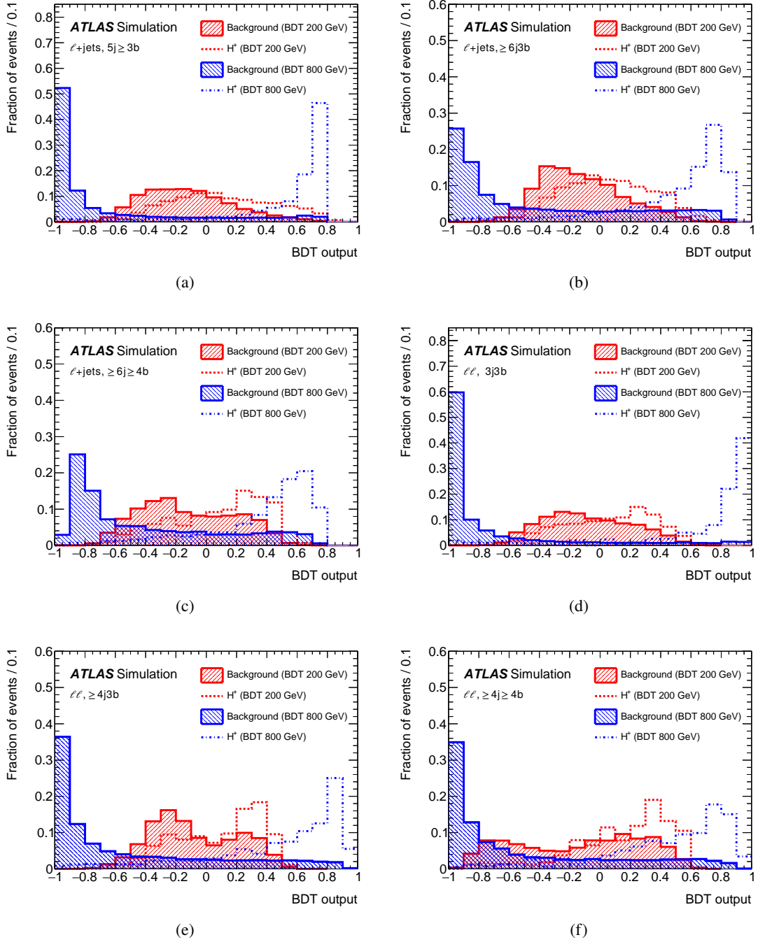
Figure 5: The expected output distributions of the BDTs employed for H^+ masses of 200 GeV and 800 GeV for SM backgrounds and H^+ signal in the three \ell +jets and the three \ell\ell SRs used in the BDT training: (a) \ell +jets final state, 5j \geq 3b , (b) \ell +jets final state, \geq 6j3b , (c) \ell +jets final state, \geq 6j \geq 4b , (d) \ell\ell final state, 3j3b , (e) \ell\ell final state, \geq 4j3b and (f) \ell\ell final state, \geq 4j \geq 4b . All distributions are normalised to unity.
