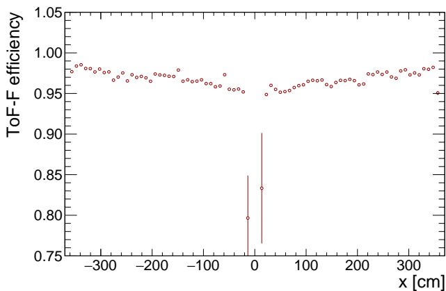
Fig. 16: Efficiency of the scintillator bars in the ToF-F wall as a function of the x -coordinate. It is clear that the efficiency drops if the bar is closer to the beamline ( x = 0 cm). This is due to an increasing track density with decreasing distance to the beam.
