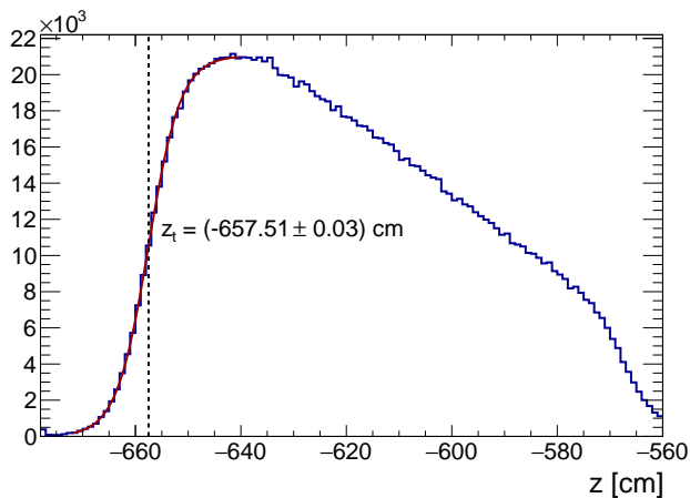
Fig. 5: The distribution of z positions of closest approach for TPC tracks extrapolated to the beam track. Only tracks whose distance to the beam track is within extrapolation uncertainty were selected. The red line shows fitted rising edge and the position of the half maximum was taken to be the target upstream z position.
