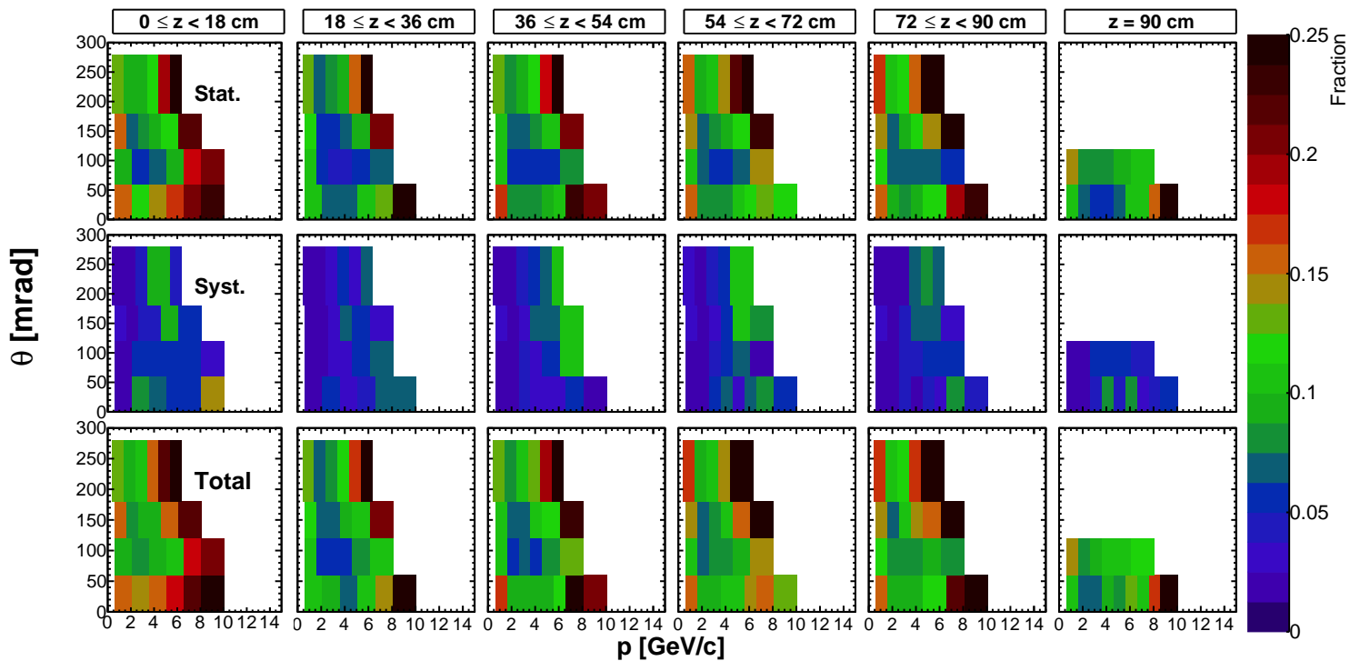
Fig. 20: Uncertainties on K^- yields shown as a function of p and \theta : statistical uncertainties (top row), total systematic uncertainties (middle row) and total uncertainties (bottom row). Each column corresponds to a different longitudinal bin.
