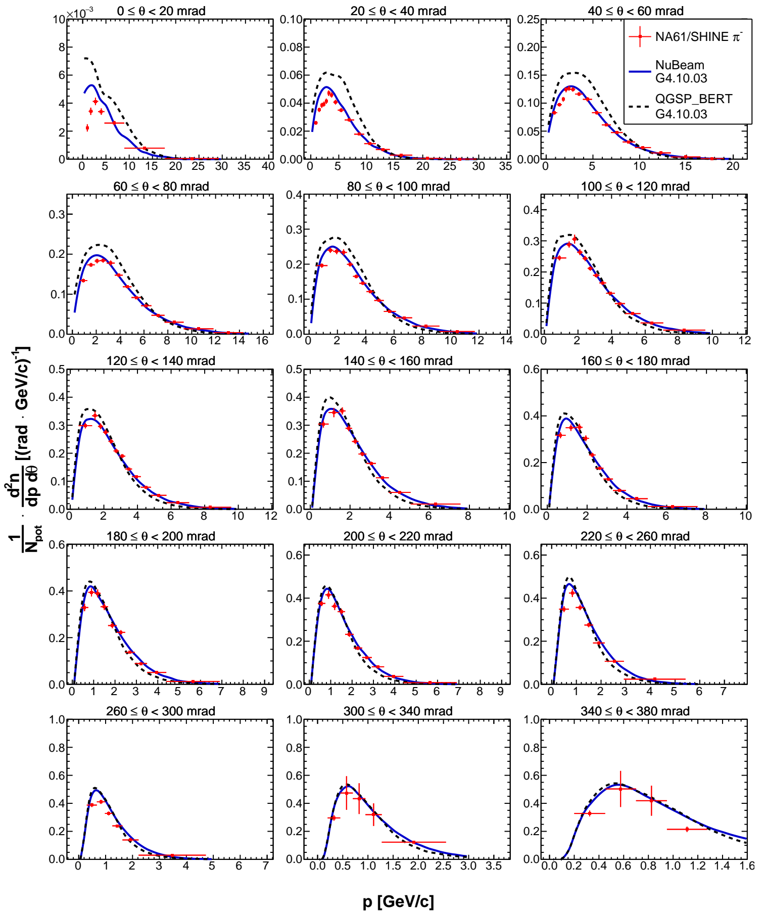
Fig. 31: Double differential yields of negatively charged pions for the third upstream longitudinal bin ( 36 \leq z < 54 cm). Vertical bars represent the total uncertainties. Predictions from the NUBEAM (solid blue line) and QGSP_BERT (dashed black line) physics lists from GEANT4.10.03 [27, 28] are overlaid on top of the data.
