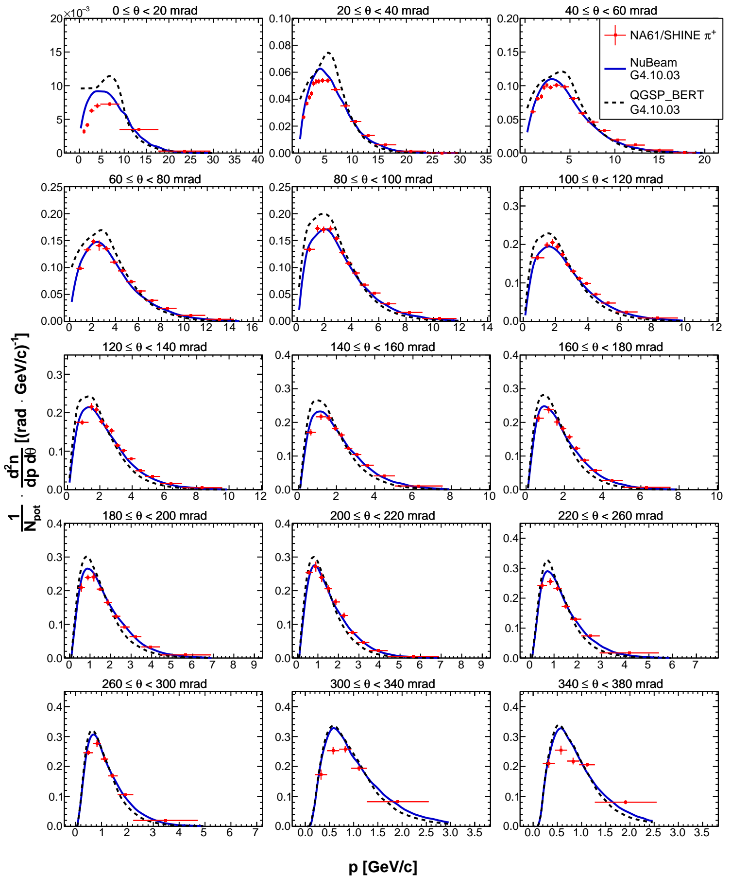
Fig. 27: Double differential yields of positively charged pions for the fifth upstream longitudinal bin ( 72 \leq z < 90 cm). Vertical bars represent the total uncertainties. Predictions from the NUBEAM (solid blue line) and QGSP_BERT (dashed black line) physics lists from GEANT4.10.03 [27, 28] are overlaid on top of the data.
