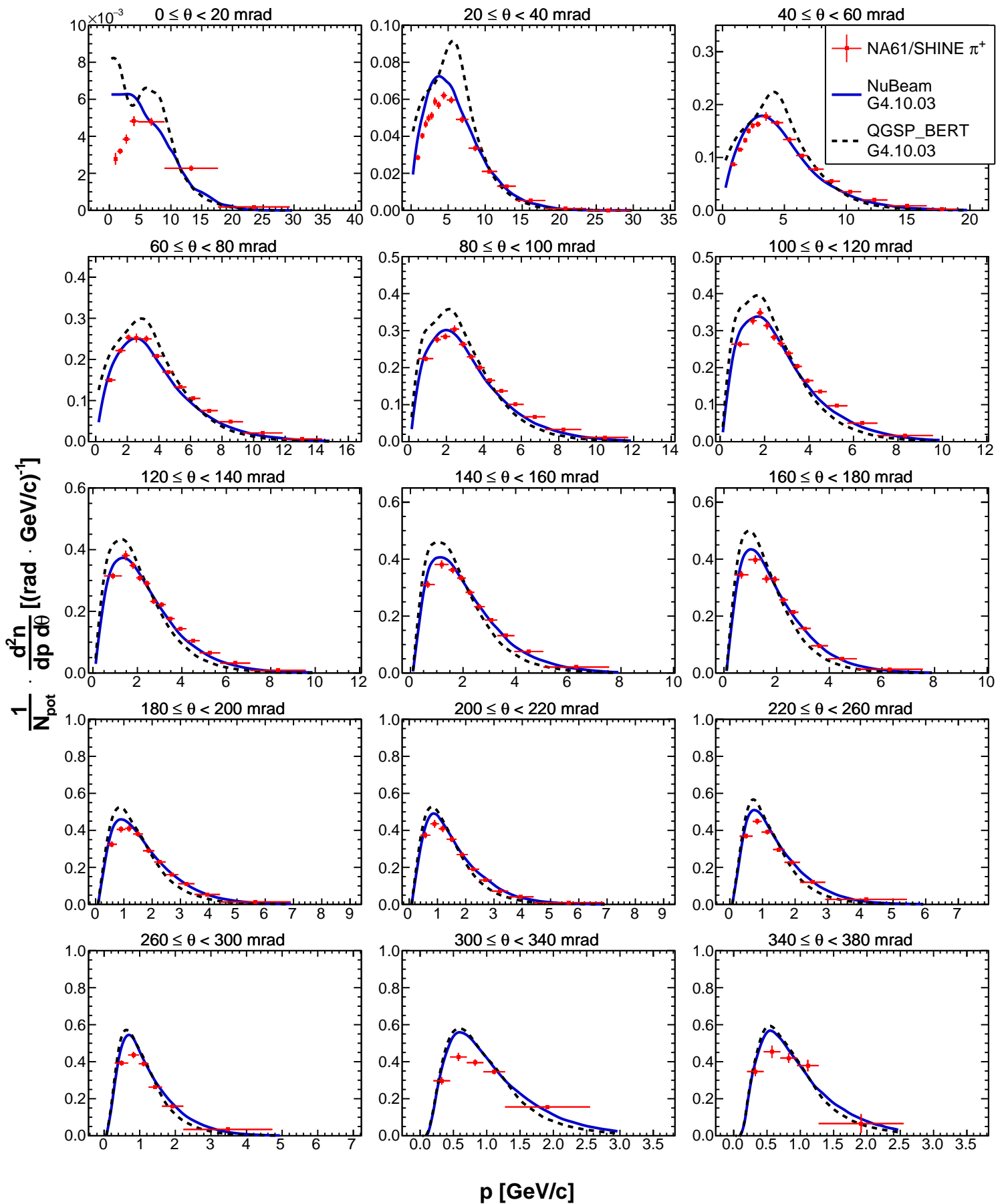
Fig. 25: Double differential yields of positively charged pions for the third upstream longitudinal bin ( 36 \leq z < 54 cm). Vertical bars represent the total uncertainties. Predictions from the NUBEAM (solid blue line) and QGSP_BERT (dashed black line) physics lists from GEANT4.10.03 [27, 28] are overlaid on top of the data.
