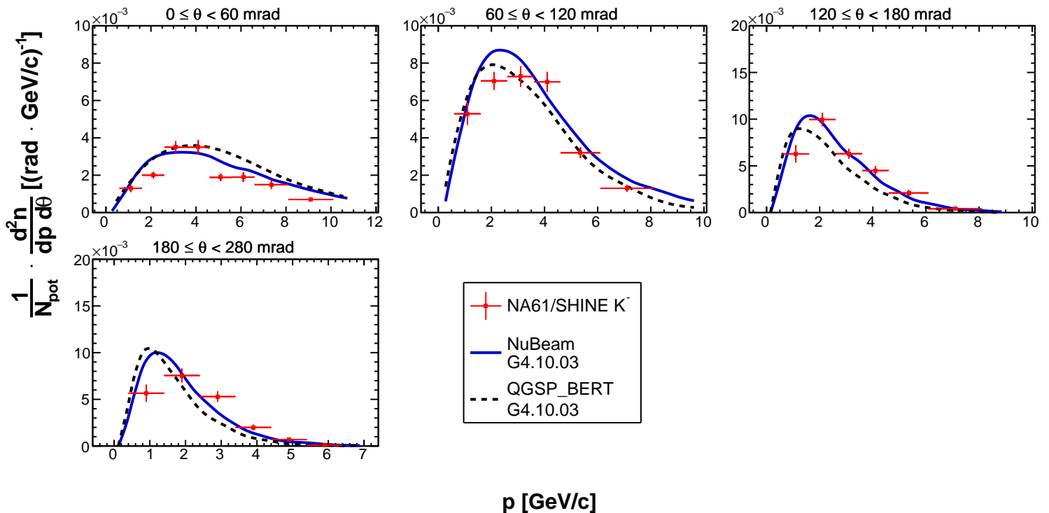
Fig. 44: Double differential yields of negatively charged kaons for the fourth upstream longitudinal bin ( 54 \leq z < 72 cm). Vertical bars represent the total uncertainties. Predictions from the NUBEAM (solid blue line) and QGSP_BERT (dashed black line) physics lists from GEANT4.10.03 [27, 28] are overlaid on top of the data.
