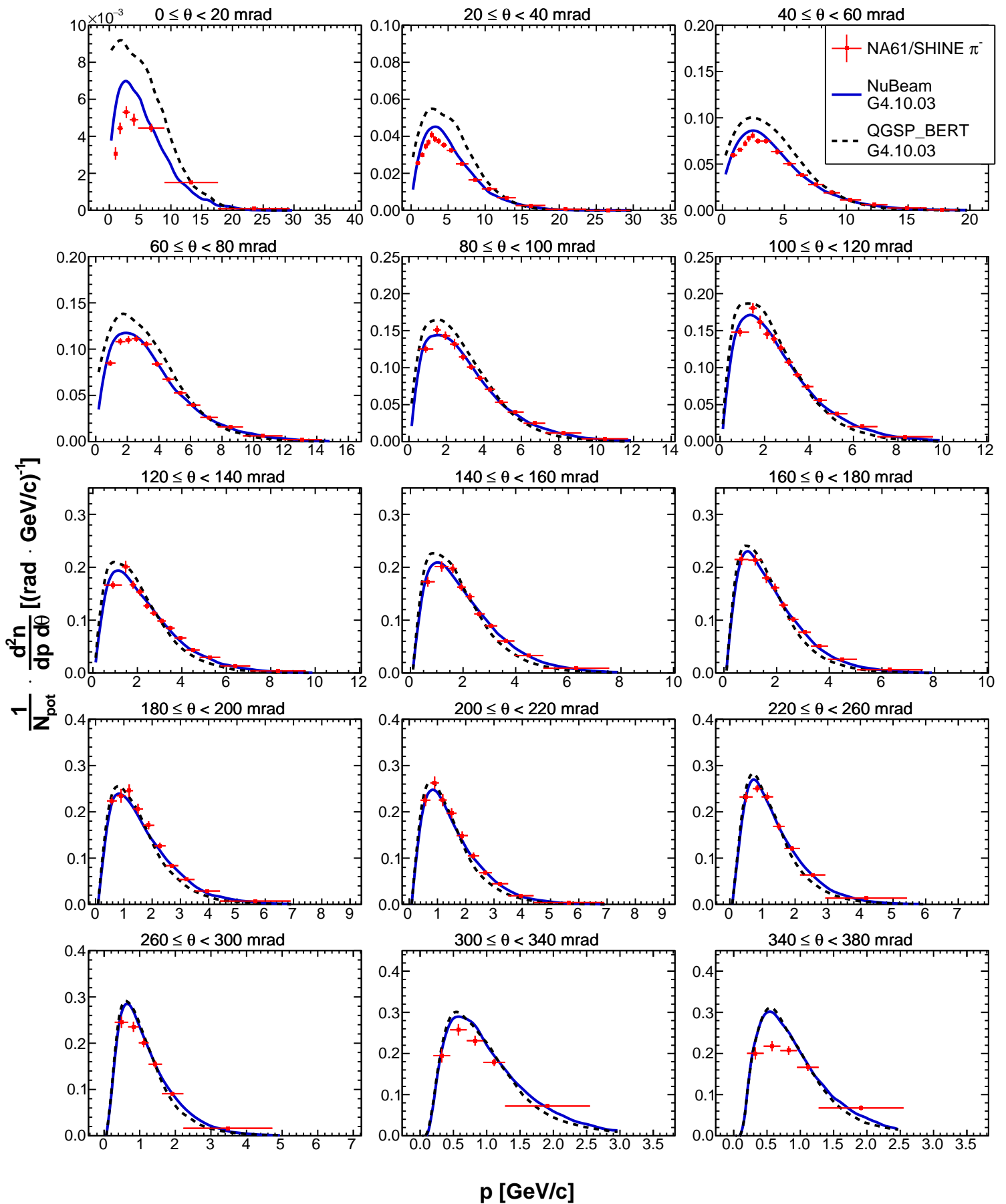
Fig. 33: Double differential yields of negatively charged pions for the fifth upstream longitudinal bin ( 72 \leq z < 90 cm). Vertical bars represent the total uncertainties. Predictions from the NUBEAM (solid blue line) and QGSP_BERT (dashed black line) physics lists from GEANT4.10.03 [27, 28] are overlaid on top of the data.
