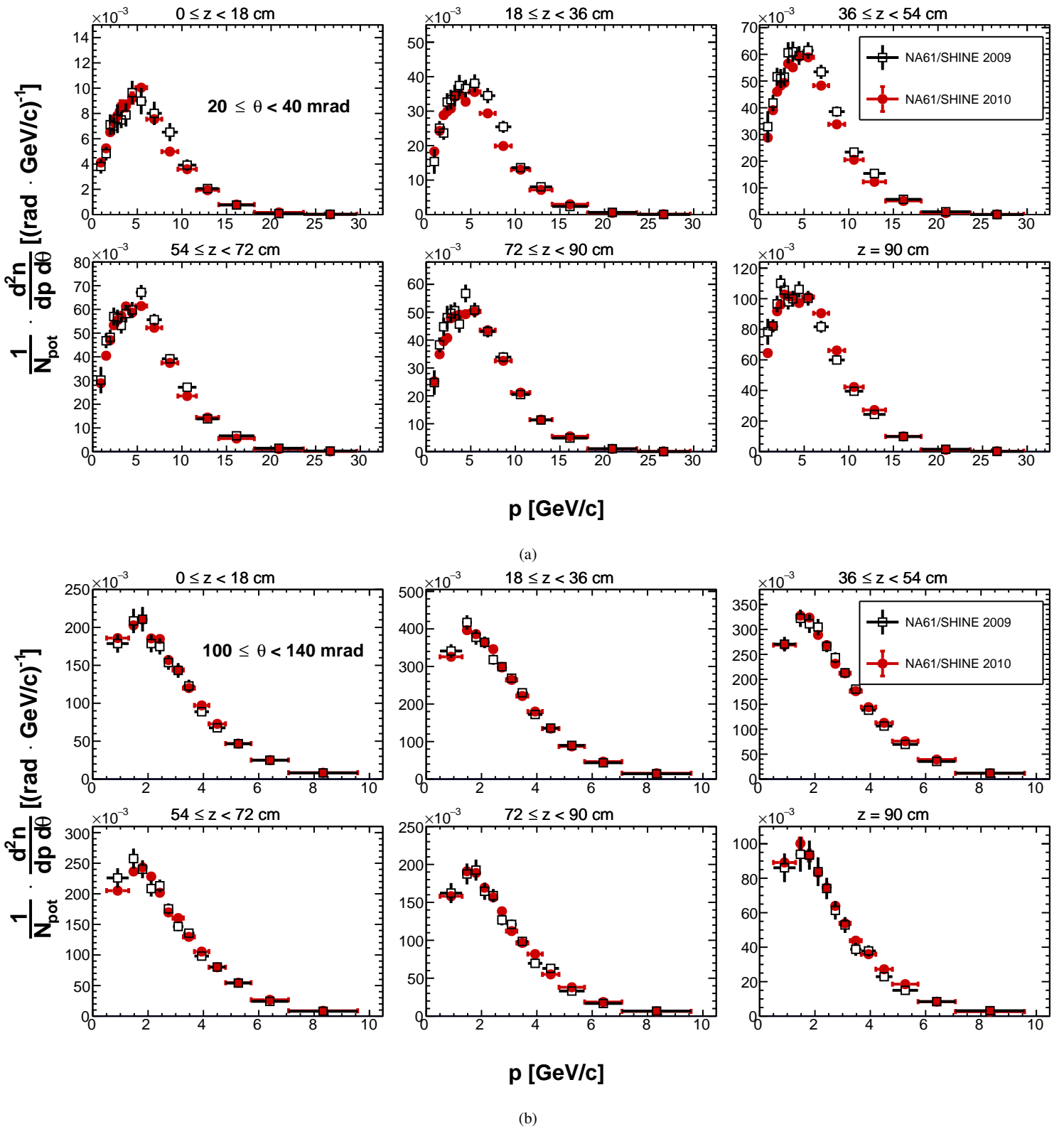
Fig. 53: Double differential yields of positively charged pions as a function of momentum for the polar angle between 20 mrad and 40 mrad (a) and between 100 mrad and 140 mrad (b). Each panel shows a different longitudinal bin. The 2009 measurements are shown in black, while the 2010 data are shown in red.
