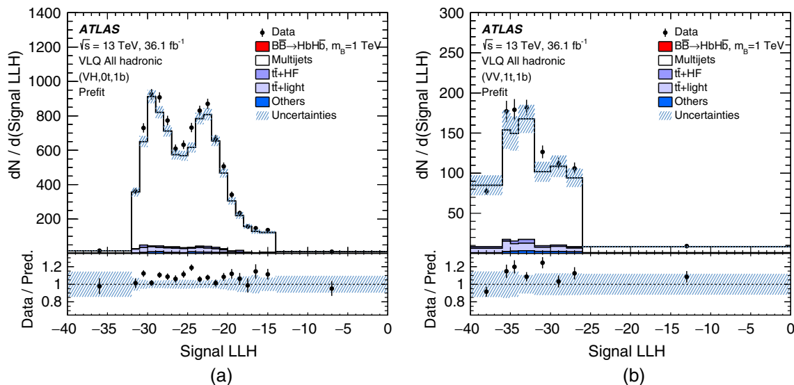
FIG. 7. Comparison between data and prediction for the signal LLH in the validation regions with two boson-tagged vRC jets, exactly one b -tagged small- R jet, and either (a) zero top-tagged vRC jets or (b) exactly one top-tagged vRC jet. The distributions show the number of events per width of 1.0 in the x axis. The hatched area represents the statistical and detector-related uncertainties of the background, added in quadrature. The deviation of the prediction from data is taken as the multijet closure uncertainty. The underflow and overflow are included in the first and last bins, respectively. These figures do not include any information from the fit described in Sec. VII, and are therefore described as “Pfit.”
