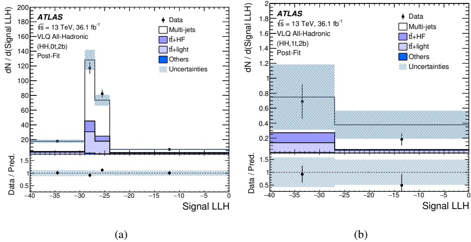
Figure 8: Comparison between data and prediction for the signal LLH in the validation regions with two Higgs-tagged \nu\text{RC} jets, exactly two b -tagged small- R jets, and either (a) zero top-tagged \nu\text{RC} jets or (b) exactly one top-tagged \nu\text{RC} jet. The distributions show the number of events per width of 1.0 in the x -axis. The hatched area represents the uncertainty on the background from statistical uncertainty and all sources of systematic uncertainty described in Section 6. The background and uncertainty take into account the constraints, pulls and correlations of the background-only fit to data of the signal regions, described in Section 7, and are therefore described as ‘Post-fit’. The underflow and overflow are included in the first and last bins, respectively.
