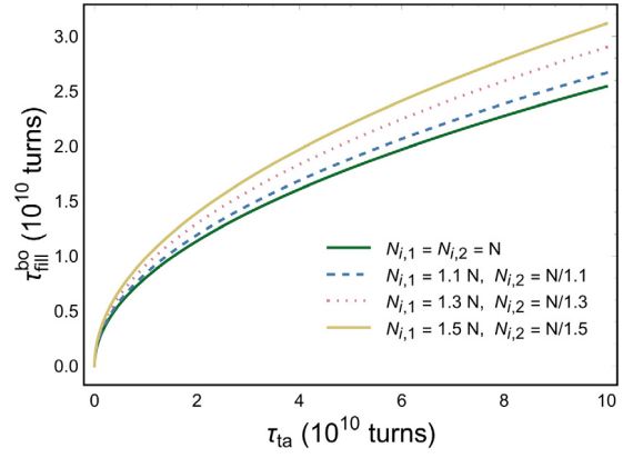
Fig. 2. Dependence of \tau_{\text{fill}}^{\text{bo}} on \tau_{\text{ta}} for equal and unequal intensities.
