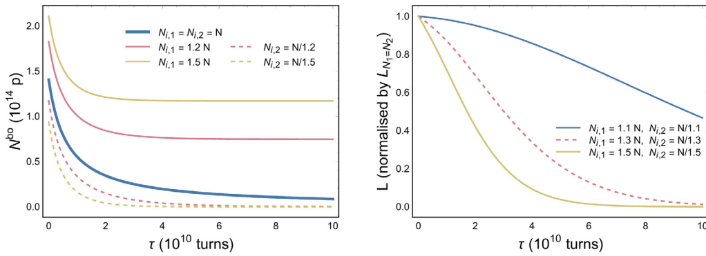
Fig. 1. Evolution of intensity (left) and luminosity (right) based on the solutions of Eqs. (12) and (13), respectively. For the plots presented here, \epsilon = 1.1 \times 10^{-24} , n_i = 1 \times 10^{11} , k_b = 1404 , which are values representative for the proton beam parameters during the Run 1 of the LHC. The luminosity evolution is normalised to the value corresponding to the solution with equal intensities. The different behaviour is clearly visible. The case with equal intensities turns out to be the best scenario as far as the luminosity is concerned.
