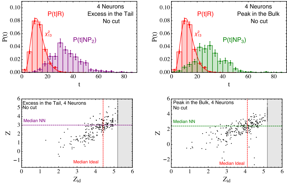
FIG. 6. Top row: Test statistic distribution in the NP 2 (left) and NP 3 (right) new physics models, compared with the reference one. The two models are defined in Eqs. (16) and (17). Bottom row: Correlation between the significances (expressed in number of \sigma 's) of our test and of the ideal test defined in Sec. II, for the NP 2 (left column) and NP 3 (right column) new physics models. The gray shaded area corresponds to the region where the ideal significance can not be computed with the number of toy data sets generated. We also show the median significance of our algorithm (Median NN) and the ideal one.
