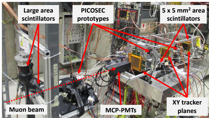
Figure 5: Photograph of the beam telescope during the beam test in May 2018. The incoming beam enters from the left side of the picture. Events are triggered either by the coincidence of two 5 \times 5 mm 2 area scintillators in anti-coincidence with a veto scintillator at the end of the telescope or by two large area scintillators in coincidence situated at the front part of the telescope. Three XY tracker planes provide tracking information of the incoming charge particles, while two MCPs give the time reference for the PICOSEC prototypes.
