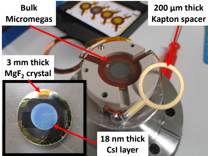
Figure 2: Photograph of the first PICOSEC prototype. The bulk Micromegas detector has a 1 cm diameter active area and its 128\ \mu\text{m} thick amplification gap is defined by six pillars, arranged in a hexagonal pattern. The mesh and anode voltages are supplied by two strip-lines onto which two coaxial cables are soldered outside the chamber. Inset: Photograph of the Cherenkov radiator and photocathode. It is composed of a \text{MgF}_2 crystal (two-inches radius and 3 mm thickness), on top of which a 5.5\ \mu\text{m} thick Chromium layer is deposited to polarize the crystal and a CsI film (12 mm-diameter and 18 nm thickness) that works as photocathode.
