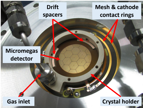
Figure 7: Photograph of the Multipad PICOSEC detector mounted on one flange of the chamber, where several components are marked: the Micromegas detector (with its 19 hexagonal pads), the drift spacers, the two contact rings for the mesh and cathode voltages; and the PEEK structure that holds a 2 inch-diameter crystal with a photocathode.
