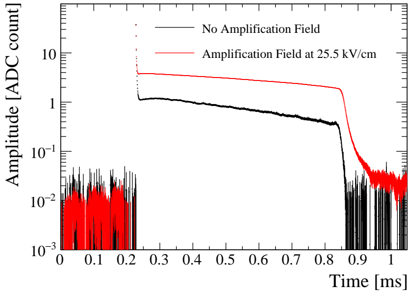
Figure 34: Sum of averaged waveforms from the 3 negative based PMTs showing the prompt and proportional scintillation components. The prominent peaks centred at around 200 \mu s correspond to the prompt scintillation in liquid (S1) and the continua extending for \sim 600 \mu s after are from the proportional scintillation in gas (S2). The higher S2 yield is clearly visible when the LEMs are polarised (red curve).
