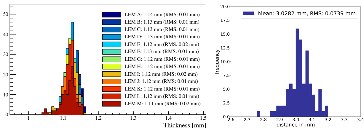
Figure 11: Left: the measured total thickness of 13 LEMs in approximately 100 points on their 50 \times 50\text{ cm}^2 surface. The measurement includes the 60\mu\text{m} of copper on both electrodes. Right: LEM anode inter-stage distance. The quoted errors represent the RMS of the distributions.
