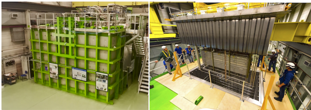
Figure 2: Pictures of the experimental setup. Left: overview of the cryostat. Right: the TPC suspended under the top-cap during insertion in the cryostat.
