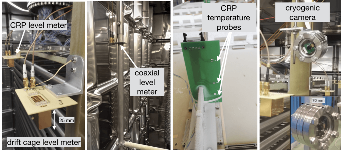
Figure 17: Pictures of some of the instrumentation in the 3 \times 1 \times 1 m 3 . From left to right: the high resolution capacitive level meters (a, b), a PCB with temperature probes to measure the gas temperature gradient near the LEMs (c) and one cryogenic camera (d).
