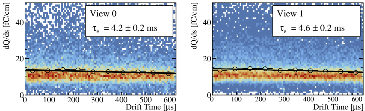
Figure 39: The scatter plot shows the collected charge per unit length in each view as a function of drift time for through-going muons. The collected charge per unit length is averaged in slices of 10 cm drift distance (corresponding to 62.5 \mu\text{s} drift time) and represented with the black markers. This distribution is fitted with an exponential function, overlaid in solid black line, the extracted electron lifetime is presented.
