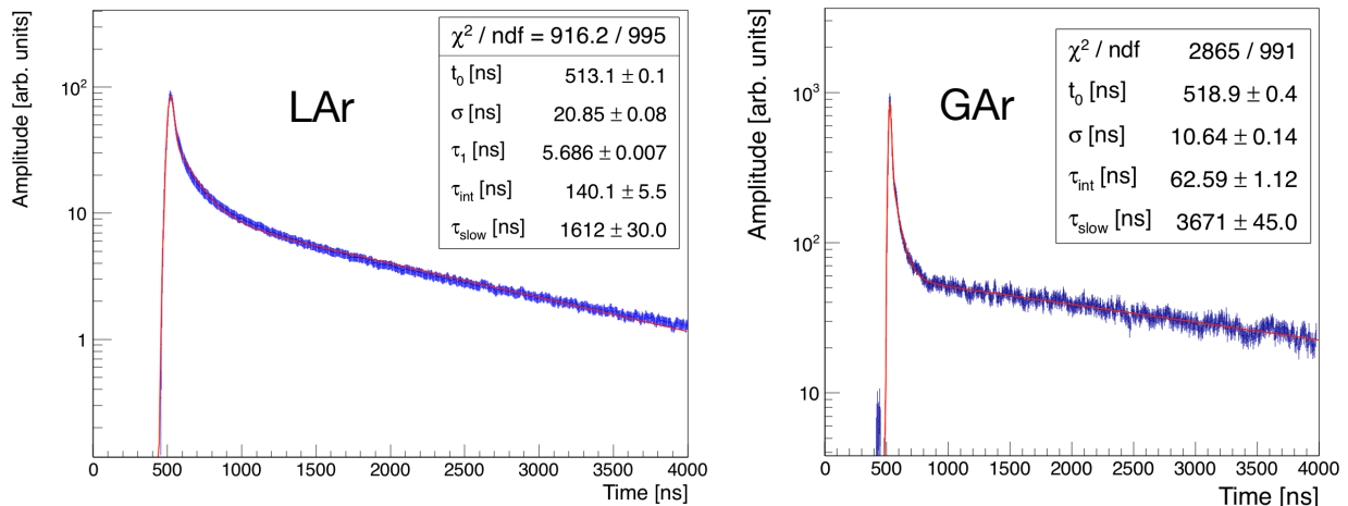
Figure 33: Average digitised signals from one PMT fitted with the function described in the text. The lifetime of the fast component is fixed to 7 ns in the fit to the gas data. Vertical scales on both plots are arbitrary and not related.
