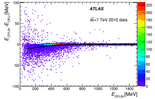
Figure 4: The absolute difference between the energies reconstructed using the optimal filtering reconstruction method with the non-iterative ( E_{\text{OFLNI}} ) and iterative ( E_{\text{OFLI}} ) signal reconstruction methods as a function of energy. The black markers represent mean values of E_{\text{OFLNI}} - E_{\text{OFLI}} per a bin of E_{\text{OFLNI}} . The parabolic correction is applied to E_{\text{OFLNI}} . The data shown uses high p_{\text{T}} ( > 20 GeV) isolated muons from \sqrt{s} = 7 TeV collisions recorded in 2010.
