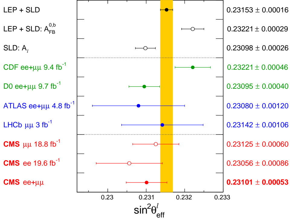
Figure 9: Comparison of the measured \sin^2 \theta_{\text{eff}}^{\ell} in the muon and electron channels and their combination, with previous LEP, SLD, Tevatron, and LHC measurements. The shaded band corresponds to the combination of the LEP and SLD measurements.
