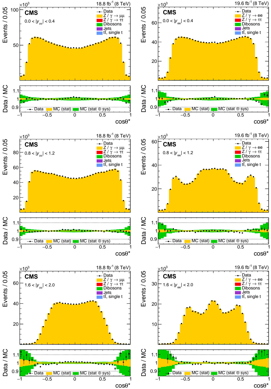
Figure 3: The muon (left) and electron (right) \cos\theta^* distributions in three representative bins in rapidity: |y_{ee}| < 0.4 (upper), 0.8 < |y_{ee}| < 1.2 (middle), and 1.6 < |y_{ee}| < 2.0 (lower). The small contributions from backgrounds are included in the predictions.
