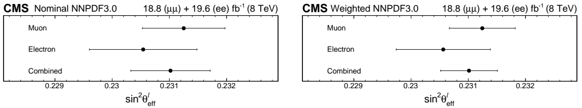
Figure 7: The extracted values of \sin^2 \theta_{\text{eff}}^l in the muon and electron channels, and their combination. The horizontal bars include statistical, experimental, and PDF uncertainties. The PDF uncertainties are obtained both without (left) and with (right) using the Bayesian \chi^2 weighting.
