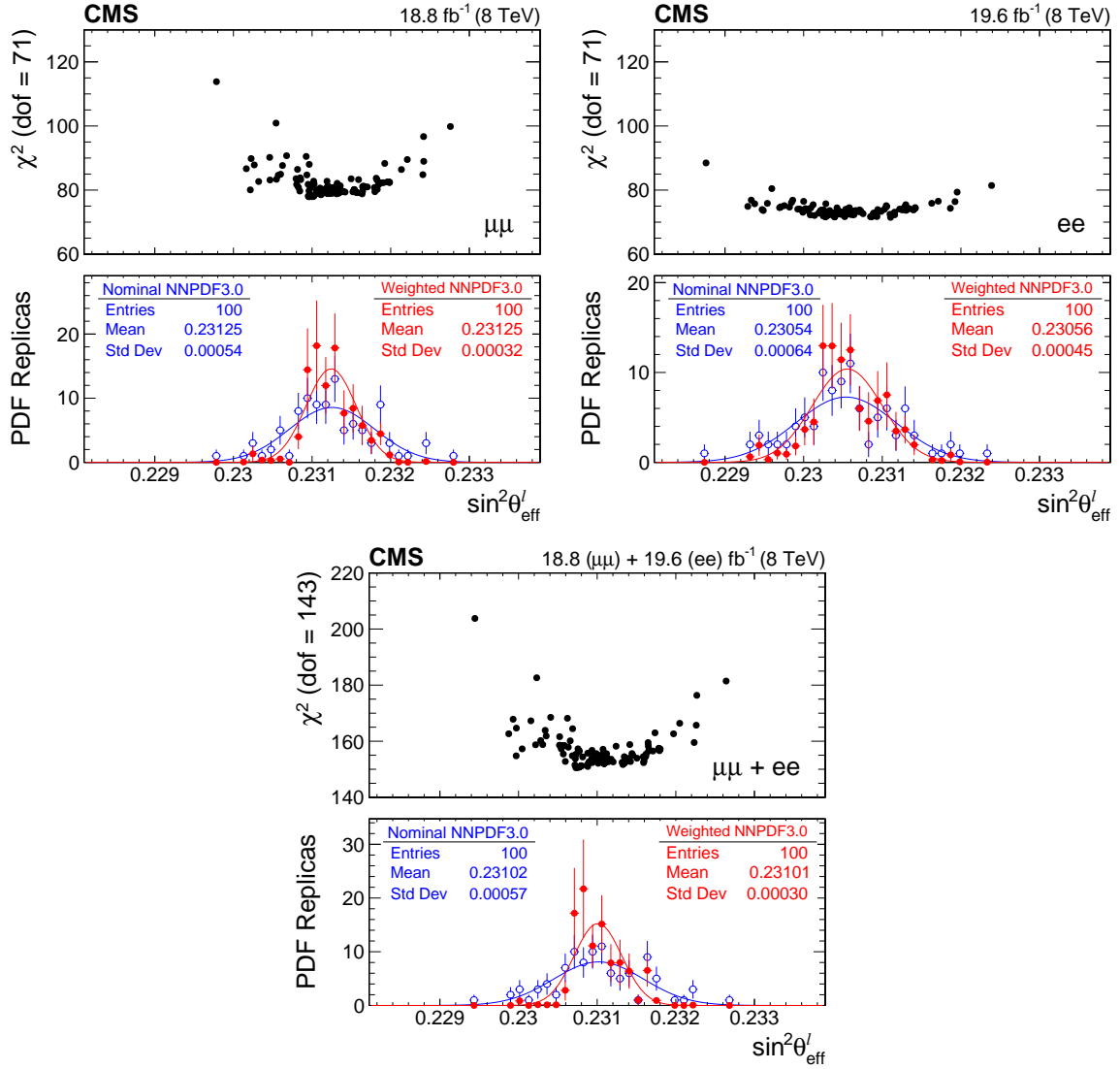
Figure 6: The upper panel in each figure shows a scatter plot in \chi^2_{\text{min}} vs. the best-fit \sin^2 \theta_{\text{eff}}^l for 100 NNPDF replicas in the muon channel (upper left), electron channel (upper right), and their combination (below). The corresponding lower panels have the projected distributions in the best-fit \sin^2 \theta_{\text{eff}}^l for the nominal (open circles) and weighted (solid circles) replicas.
