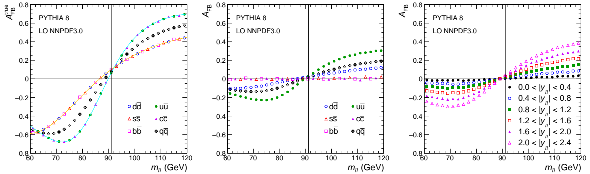
Figure 1: The dependence of A_{\text{FB}} on m_{\ell\ell} in dimuon events generated using PYTHIA 8.212 [16] and the LO NNPDF3.0 [17] PDFs for dimuon rapidities of |y_{\ell\ell}| < 2.4 . The distributions for the total production ( q\bar{q} ) and the different channels are given on the left, overlaid with results based on Eq. (6), using the definition of A_{\text{FB}}^{\text{true}}(m_{\ell\ell}) for the known quark direction. The middle panel gives the diluted A_{\text{FB}} using instead the direction of the dilepton boost, and the right panel shows the diluted A_{\text{FB}} in |y_{\ell\ell}| bins of 0.4 for all channels.
