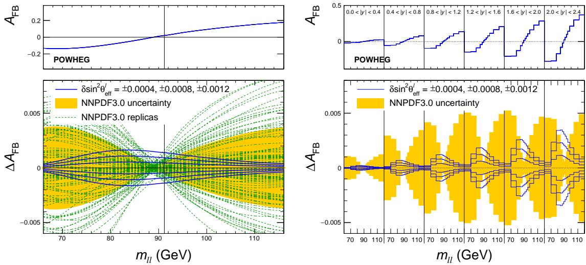
Figure 5: Distribution in A_{\text{FB}} as a function of dilepton mass, integrated over rapidity (left), and in six rapidity bins (right) for \sin^2 \theta_{\text{eff}}^\ell = 0.23120 in POWHEG. The solid lines in the bottom panel correspond to six changes at \sin^2 \theta_{\text{eff}}^\ell around the central value, corresponding to: \pm 0.00040 , \pm 0.00080 , and \pm 0.00120 . The dashed lines refer to the A_{\text{FB}} predictions for 100 NNPDF3.0 replicas. The shaded bands illustrate the standard deviation in the NNPDF3.0 replicas.
