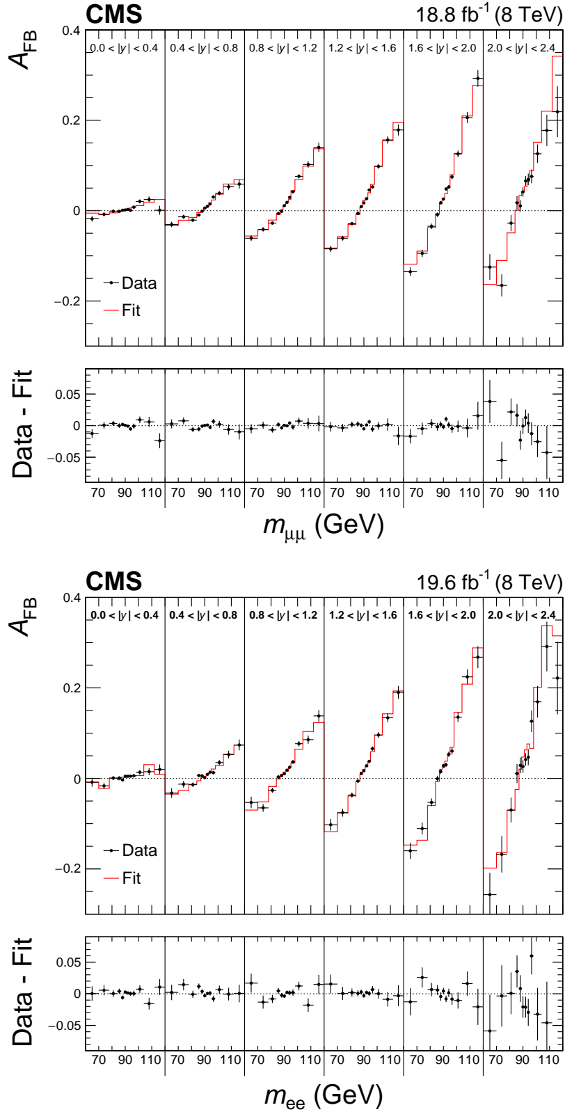
Figure 4: Comparison between data and best-fit A_{\text{FB}} distributions in the dimuon (upper) and dielectron (lower) channels. The best-fit A_{\text{FB}} value in each bin is obtained via linear interpolation between two neighboring templates. Here, the templates are based on the central prediction of the NLO NNPDF3.0 PDFs. The error bars represent the statistical uncertainties in the data.
