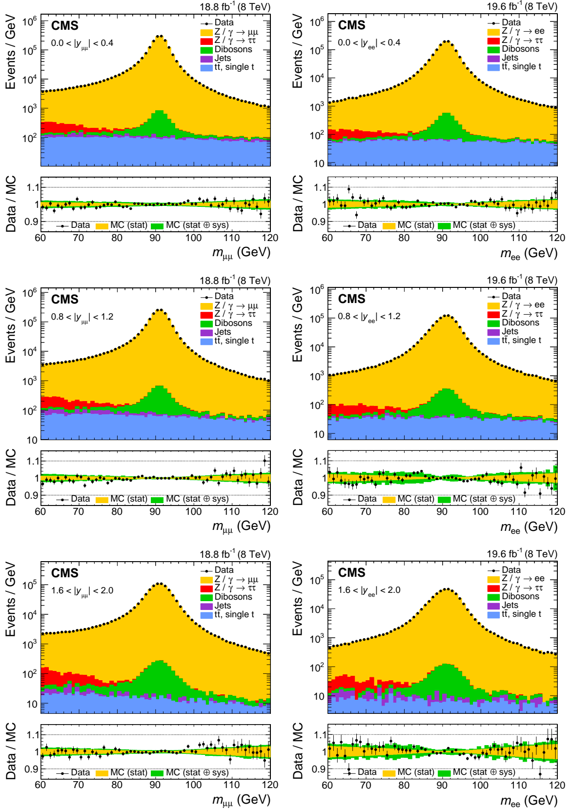
Figure 2: Dimuon (left) and dielectron (right) mass distributions in three representative bins in rapidity: |y_{ee}| < 0.4 (upper), 0.8 < |y_{ee}| < 1.2 (middle), and 1.6 < |y_{ee}| < 2.0 (lower).
