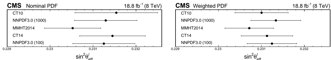
Figure 8: Extracted values of \sin^2 \theta_{\text{eff}}^\ell from the dimuon data for different sets of PDFs with the nominal (left) and \chi^2 -reweighted (right) replicas. The horizontal error bars include contributions from statistical, experimental, and PDF uncertainties.
