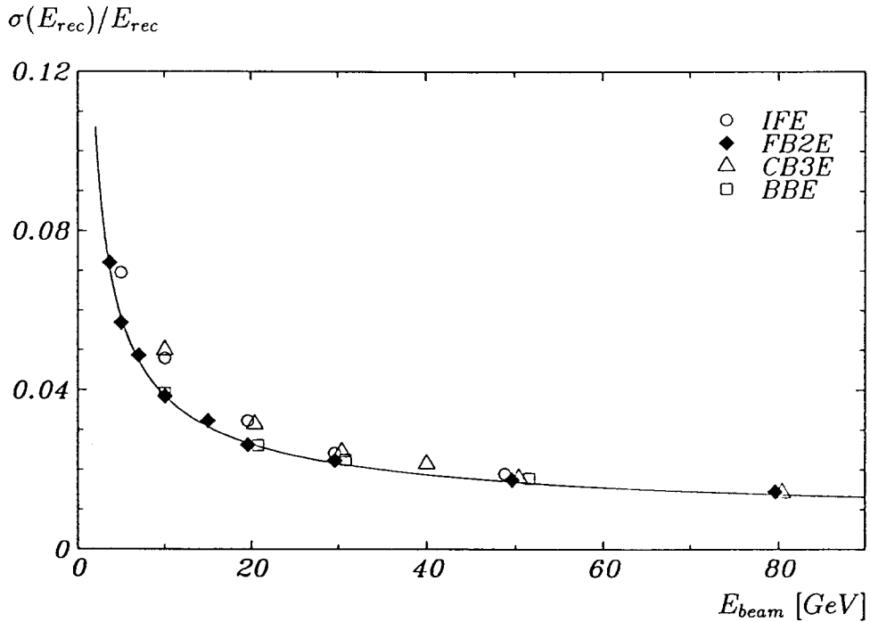
Figure 19: Energy resolution for the various calorimeter wheels as a function of the beam energy.
