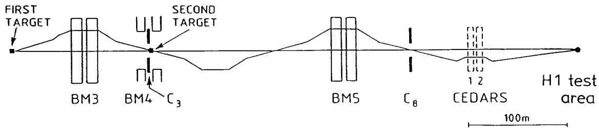
Figure 4: Schematic view of the optics of the H6 beam in the vertical plane.
