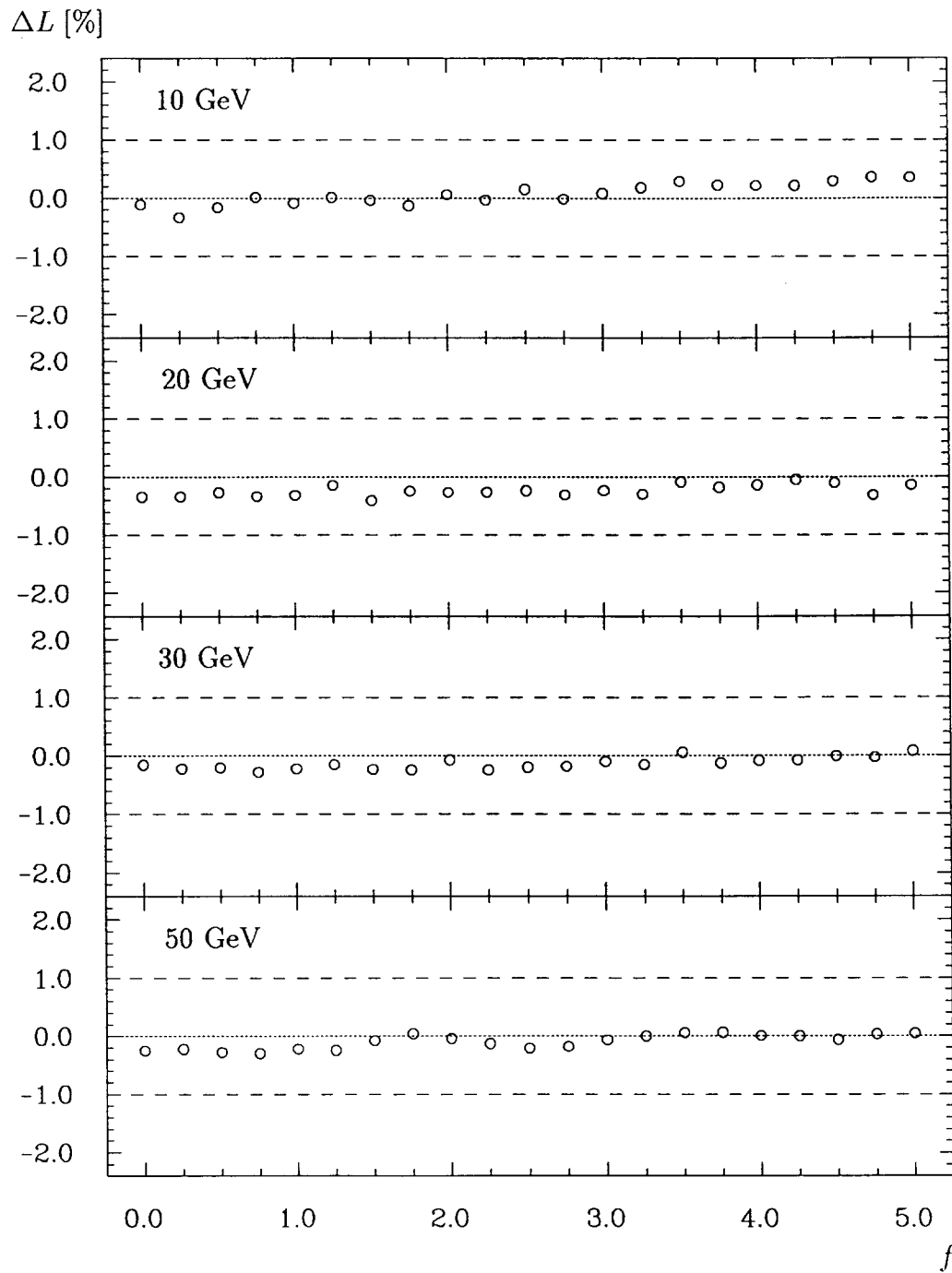
Figure 11: Relative deviations \Delta L (eq. (7)) for various beam energies entering a BBE module as a function of the noise threshold f (eq. (4)). The dashed lines mark the \pm 1\% range. The statistical errors are smaller than the symbol size.
