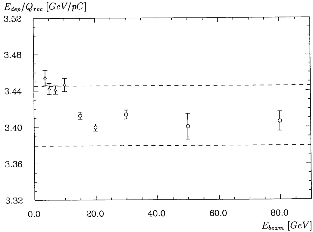
Figure 18: Linearity of the calorimeter signal in a FB2E module as measured by the ratio of deposited energy, calculated by simulations, and reconstructed charge as a function of the beam energy. The values for E_{beam} \leq 10 GeV ( \triangle ) have been measured by a different set-up of the beam. The dashed lines mark the \pm 1\% range.
