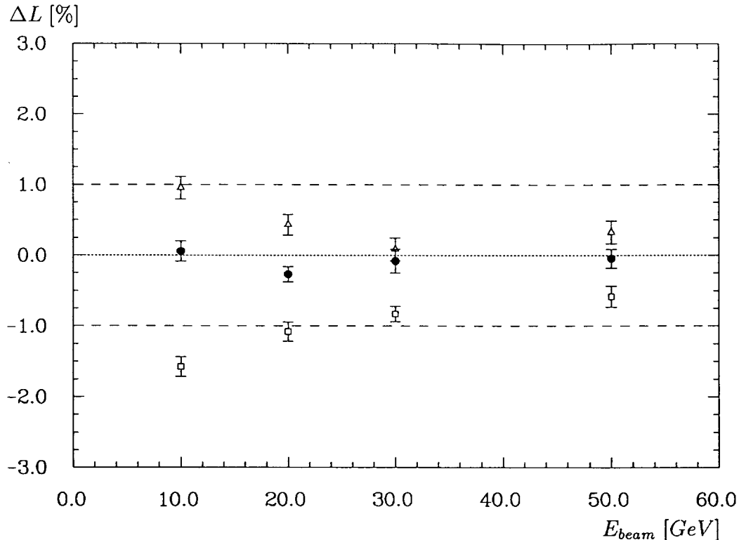
Figure 12: Relative deviations \Delta L (eq. (7)) for various amounts of inactive material in front of the calorimeter ( 0.66X_0 ( \Delta ), 1.06X_0 ( \bullet , nominal), 1.30X_0 ( \square )) as a function of the energy of particles entering a BBE module. The dashed lines mark the \pm 1\% range.
