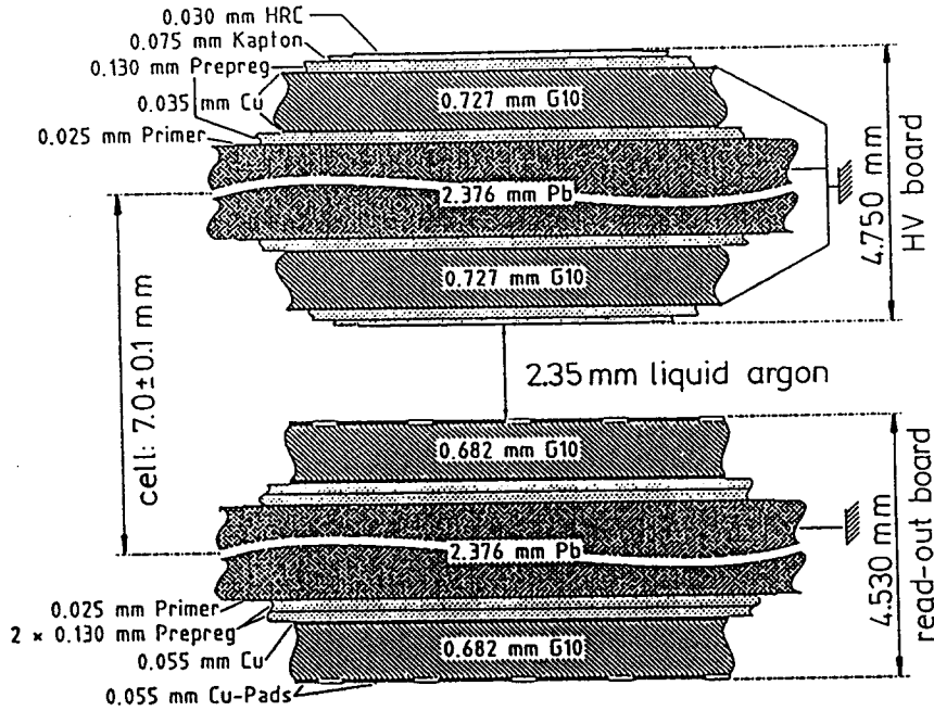
Figure 2: Schematic view of the electromagnetic sampling structure in the FB2E wheel (not to scale).
