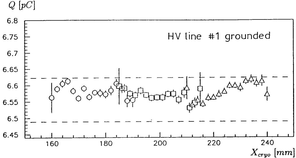
Figure 17: Calorimeter signal in a scan measured in a FB2E module with one grounded high voltage line. All data with the same symbol belong to one cryostat position, the real particle impact point was determined by using the MWPC2 (see section 2.1). The dashed lines mark the \pm 1\% range.
