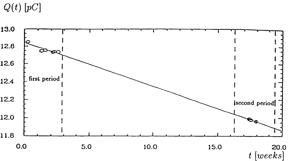
Figure 7: Time dependent decrease of the measured charge Q for 30 GeV electrons during the time of the IF measurements, fitted by a straight line.
