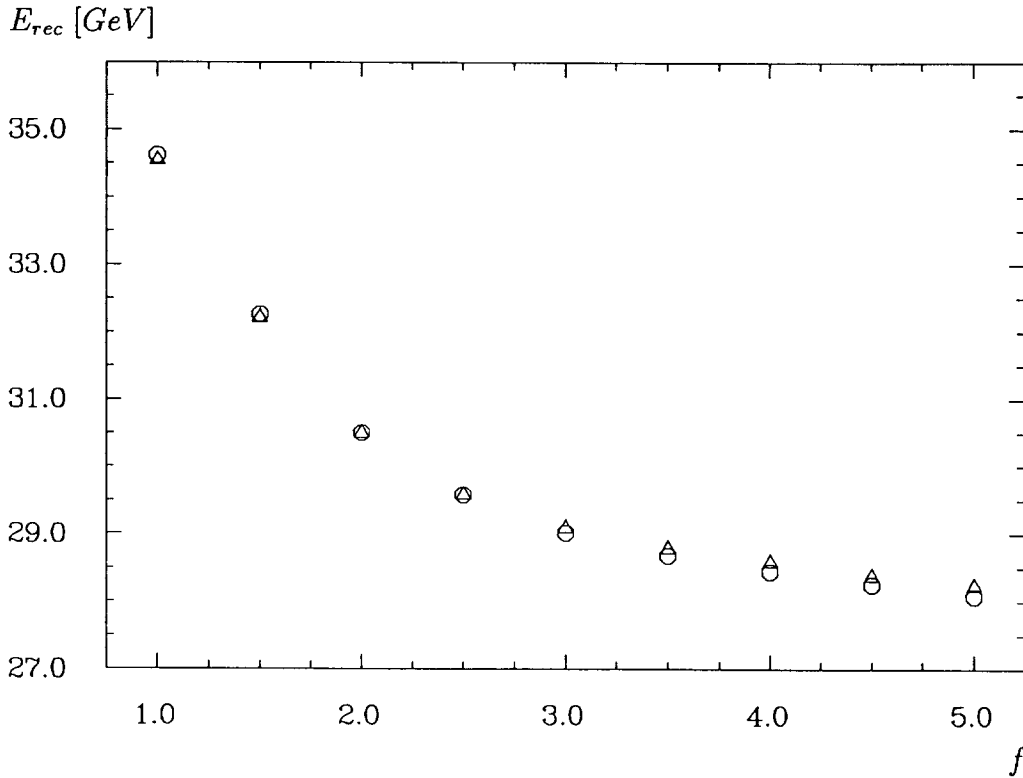
Figure 10: Reconstructed energies as function of the noise threshold f (see equation (4) for definition) for measured ( \circ ) and simulated ( \triangle ) events with 30 GeV electrons entering an IFE module. The statistical errors are smaller than the symbol size.
