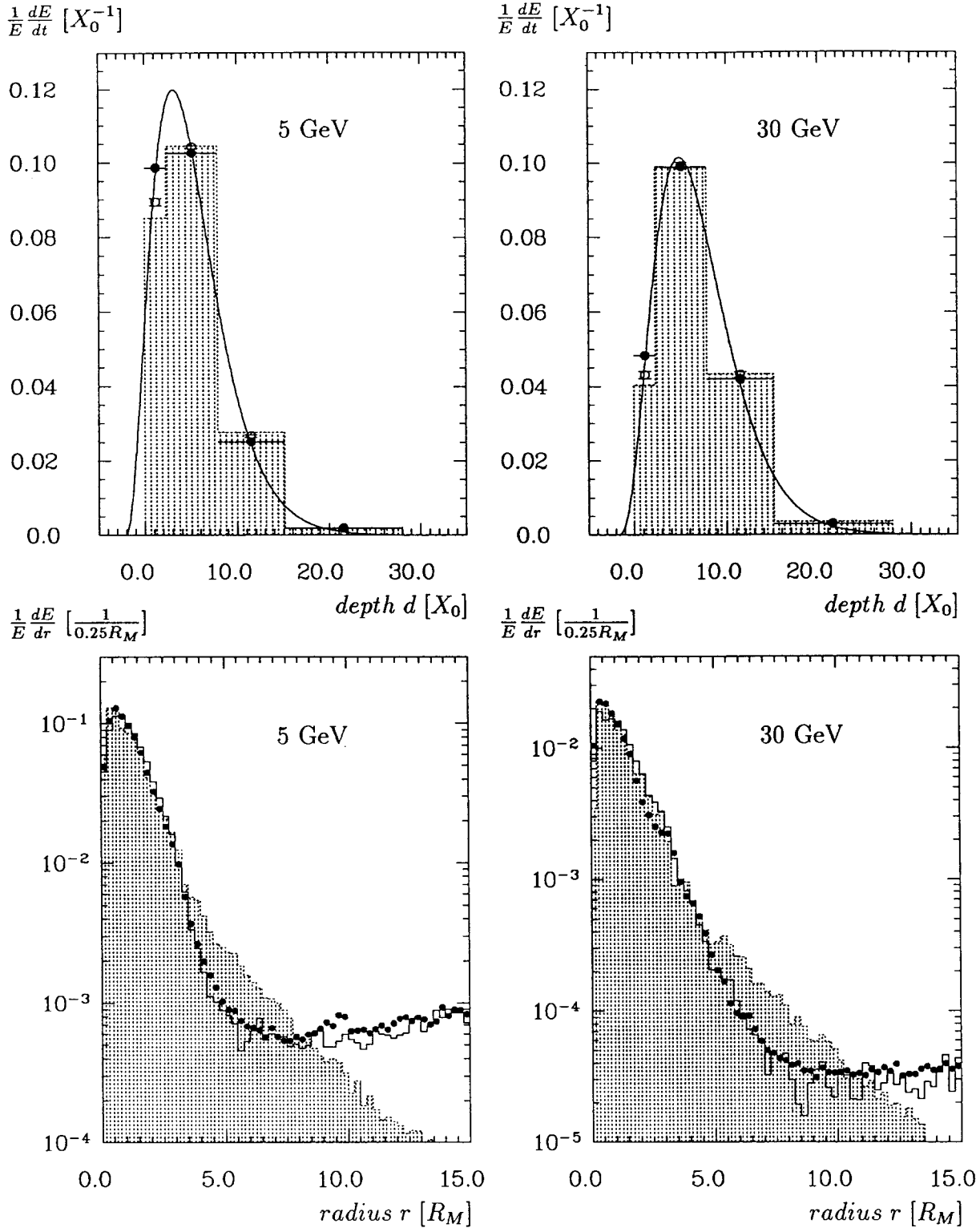
Figure 13: Longitudinal (upper pictures) and lateral (lower pictures) shower profiles as reconstructed for 5 and 30 GeV in the IFE calorimeter for data ( \bullet ), GEANT simulations including noise ( \circ or histogram) and pure GEANT simulations (hatched histogram). The lines indicate fits to the longitudinal shower profiles.
