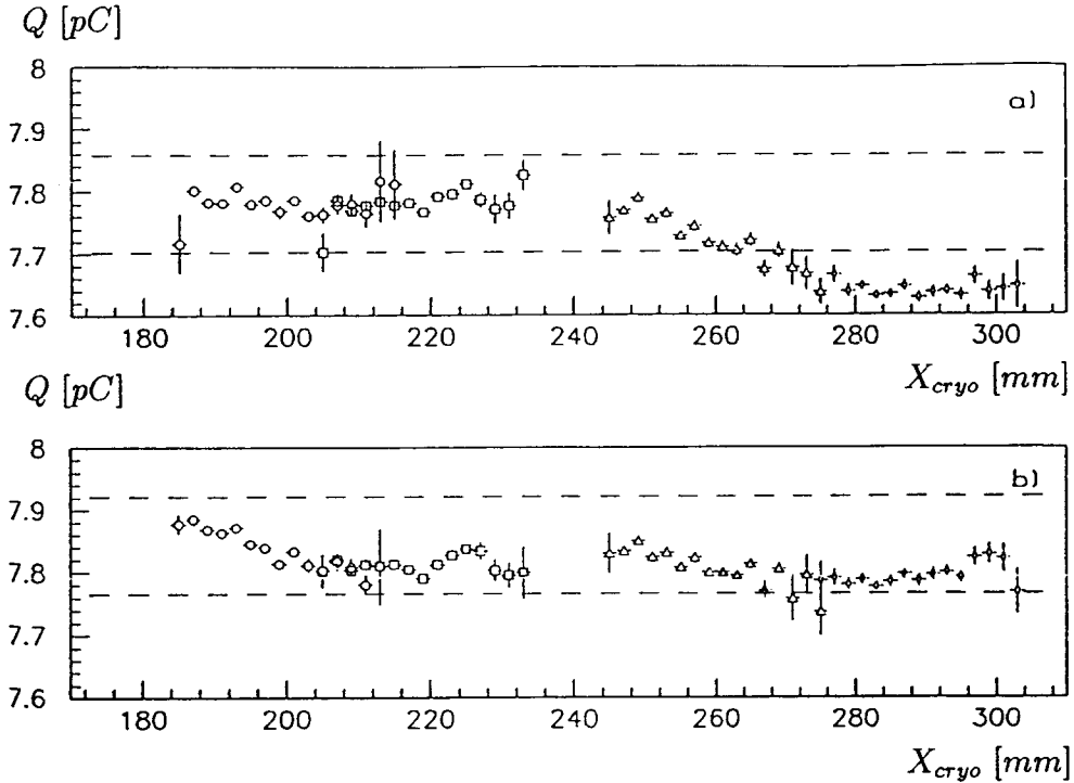
Figure 14: Calorimeter signal in a scan, where the impact points of the beam particles moved in z -direction (see fig. 1) across a FB2E module, without gap width correction (a)) and with gap width correction (b)). The center steel plate (see chapter 1) is close to X_{\text{cryo}}=280 mm. All data with the same symbol belong to one cryostat position, the real particle impact point was determined by using the MWPC2 (see section 2.1). The dashed lines mark the \pm 1\% range.
