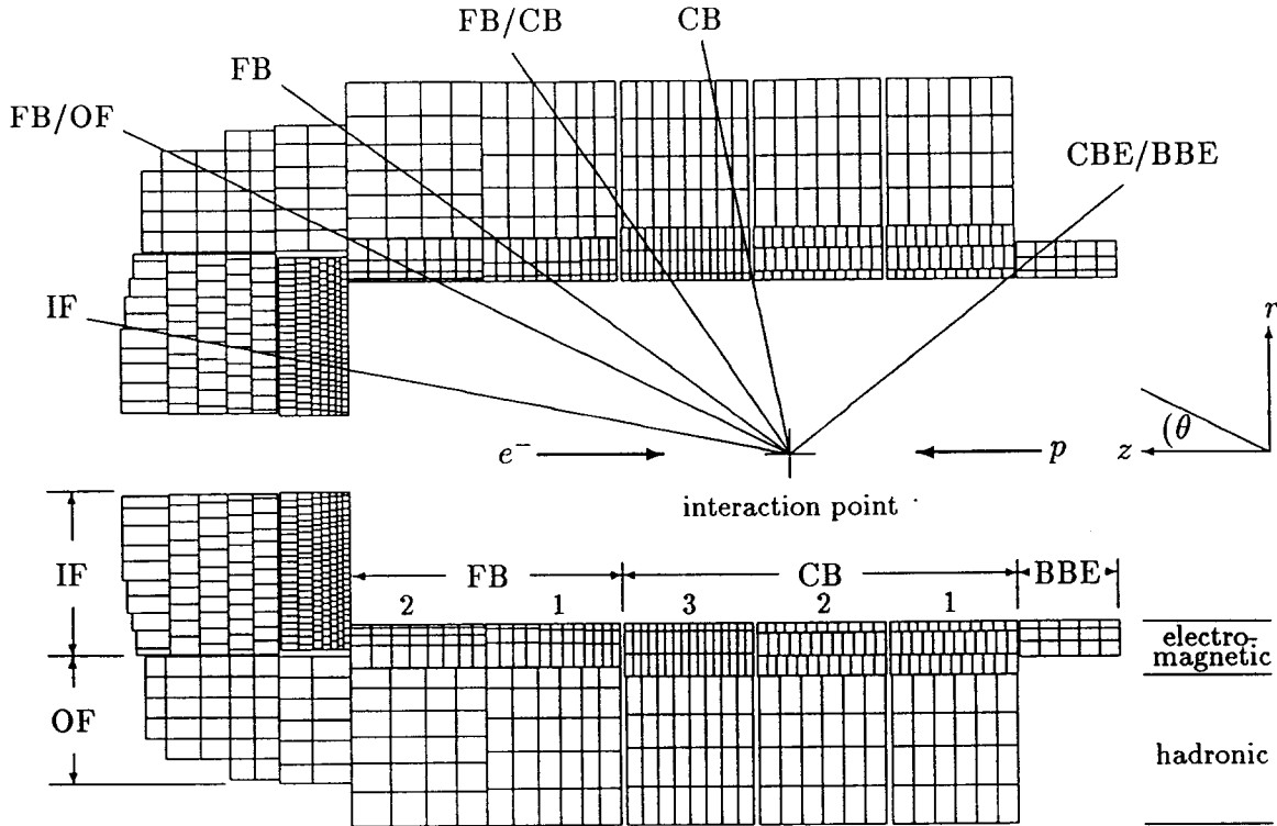
Figure 1: Schematic view of the wheel and cell structure of the H1 LAr calorimeter. The lines from the interaction point indicate the nominal beam directions in the test set-up for the different calibration measurements discussed here. For spatial scans the beam was shifted perpendicular to the lines drawn in a way that the impact point of the particles moved either in z -direction or perpendicular to the r - z -plane.
