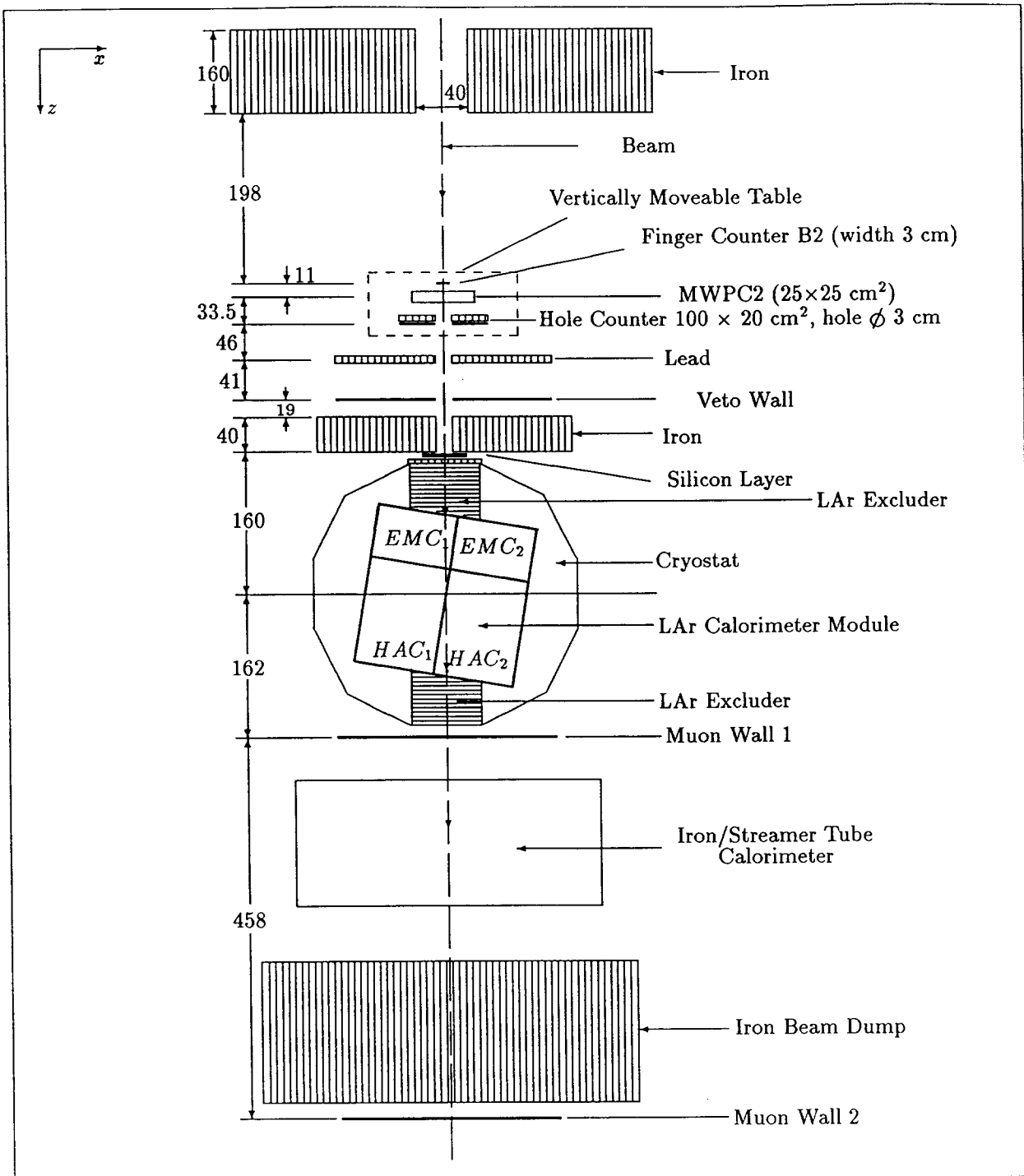
Figure 5: Schematic view on the set-up in H1 test area at the H6 beam (dimensions in cm).
