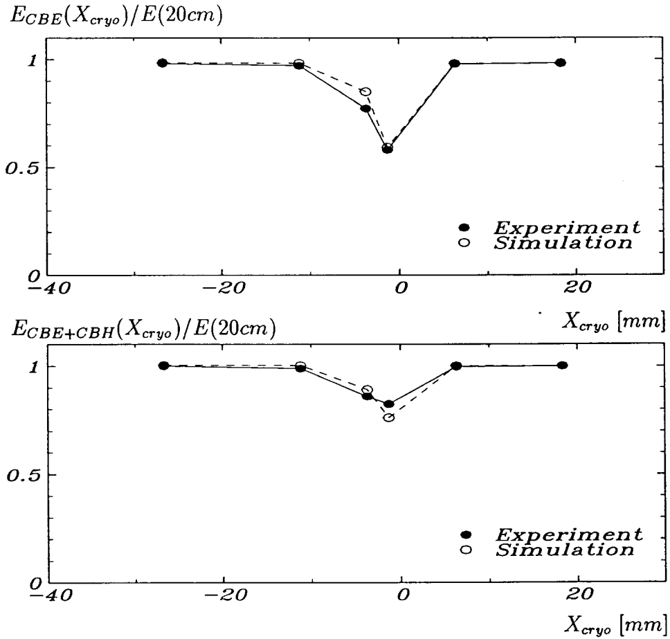
Figure 16: Calorimeter signal of 30 GeV electrons in a scan across the most unfavourable z -crack between the CB2 and the CB3 modules (see fig. 1). The upper picture shows the energy reconstructed in the electromagnetic module, while in the lower picture also the energy deposition in the hadronic part is considered. The reconstructed energies are normalized and compared with the energy measured at a distance of 20 cm from the crack ( E(20\text{cm}) ). The simulation, based on parametrized electromagnetic showers (see section 2.4), gives a good description of the data and was used to develop a correction for the H1 shower reconstruction program.
