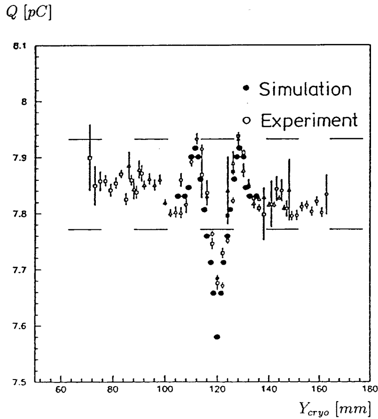
Figure 15: Calorimeter signal of a FB2E module in a scan, where the impact points of the beam particles moved perpendicular to the r - z -plane (see fig. 1) across a FB2E module. The upper picture shows the whole scan with the crossing of two rods ( Y=-110 mm, Y=120 mm). All data with the same symbol belong to one beam setting with the bending magnet BM9, the real particle impact point was determined by using the MWPC2 (see section 2.1). The lower picture shows a comparison with EGS4 simulations in the surrounding of the second rod. The dashed lines mark the \pm 1\% range.
