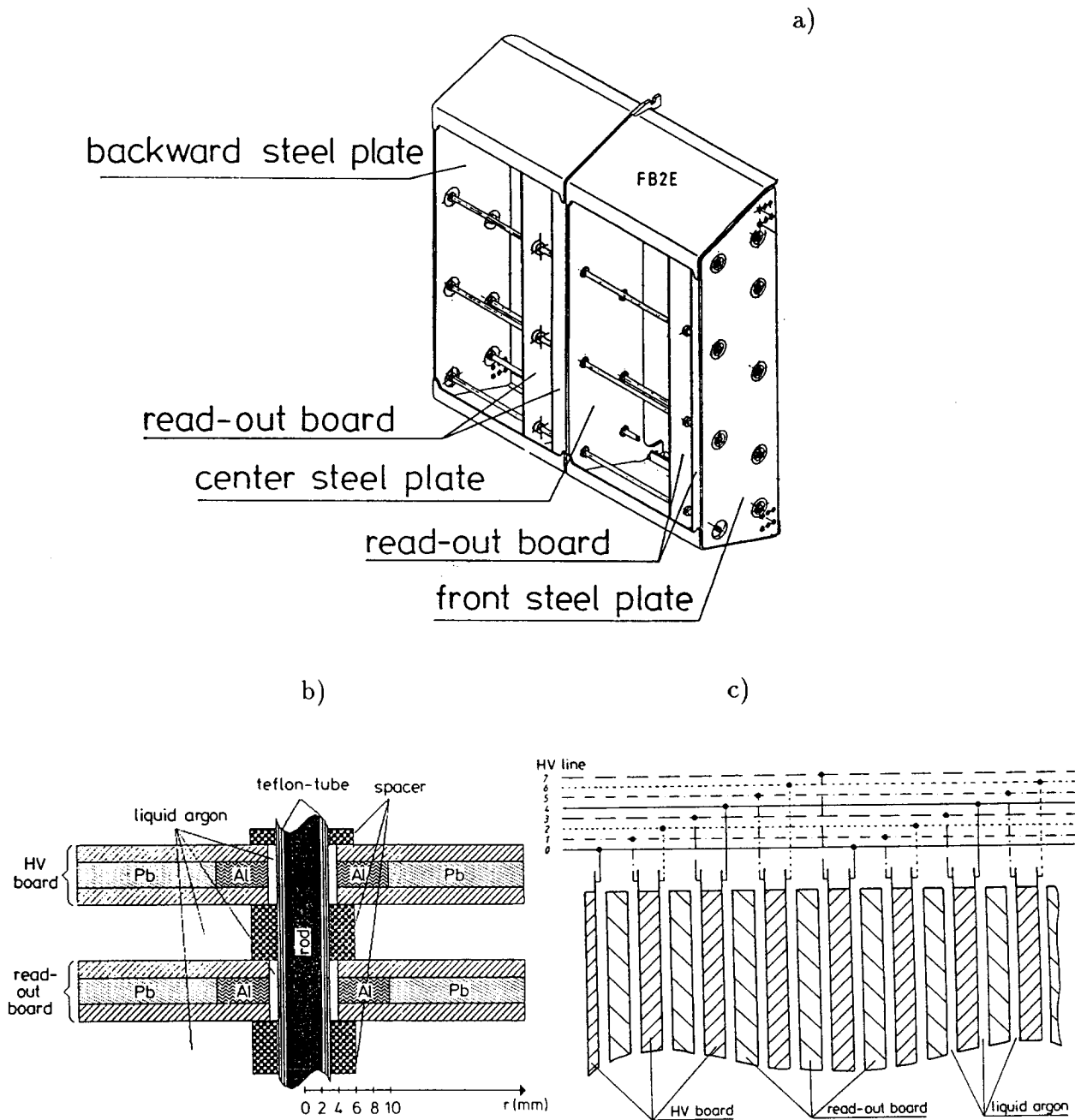
Figure 3: Design characteristics of a FB2E module: a) view of the support structure, b) absorber board construction in the surrounding of the steel rods, c) high voltage distribution.
