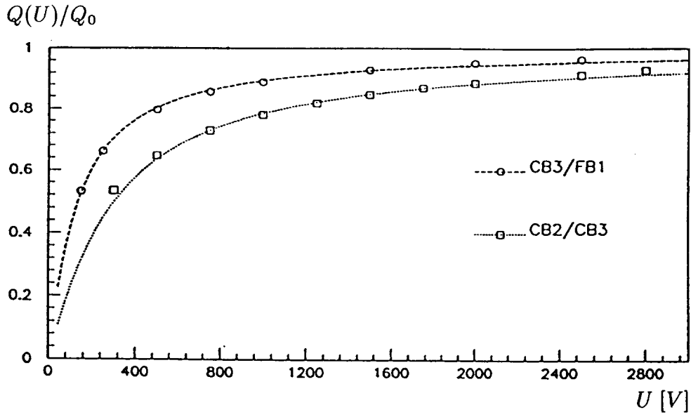
Figure 6: Measured charge Q as function of the high voltage U applied to the calorimeters, normalized to the extrapolated plateau charge Q_0 for two different module configurations. The curves are fits based on eq. (1).
