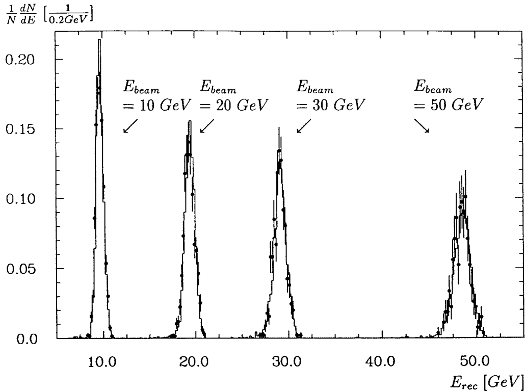
Figure 8: Distribution of reconstructed energies E_{rec} for measured (histogram) and simulated (•) events in a BBE module for the beam energies 10, 20, 30 and 50 GeV.
