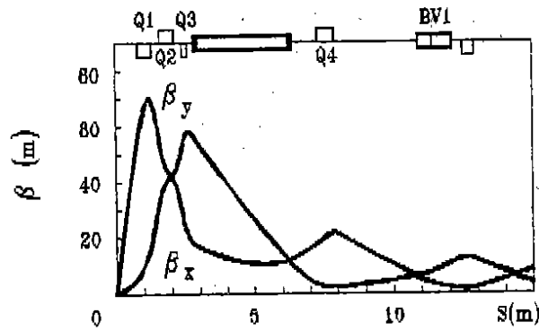
Fig. 6. Lattice functions in interaction region.
