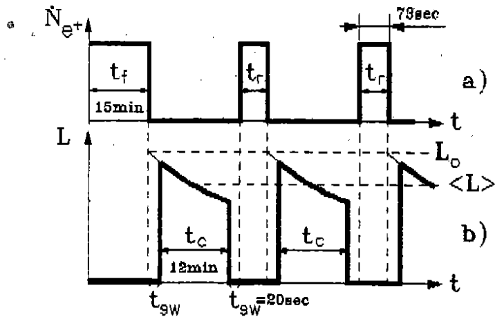
Fig. 3. The injection complex cyclogram: positron flux N_{e^+} from the injection complex (a) and the luminosity variation (b). t_f - the positron "full-fill" time; t_r - the refilling time; t_c - the counting time; t_{sw} - the detector switch on/off time; \langle L \rangle - the average luminosity.
