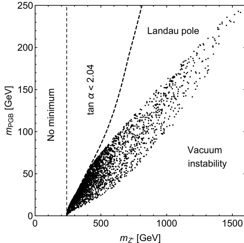
Figure 5: Allowed mass ranges for the new scalar and Z' particles in the Gildener–Weinberg scenario B which are perturbatively stable up to the Planck scale.
