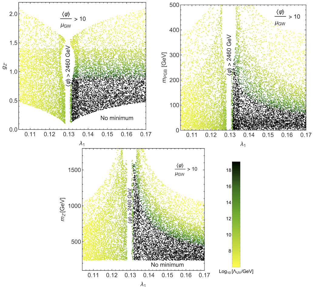
Figure 4: Largest possible UV scales in the GW scenario B of the Hempfling model where the Higgs is not the PGB particle. A random set of 12000 dials of (\lambda_1, g_{Z'}) in the realm \lambda_1 \in [0.1, 0.17] and g_{Z'} \in [0, \pi] were performed, tested for perturbative viability and the UV breakdown scale of every point computed. The non-smooth jump at \lambda_1 \sim 0.13 from a UV-cutoff at the Planck scale to around 10^{12} GeV is due to the onset of vacuum instability (negative \lambda_1 or \lambda_2 ) at that intermediate scale.
