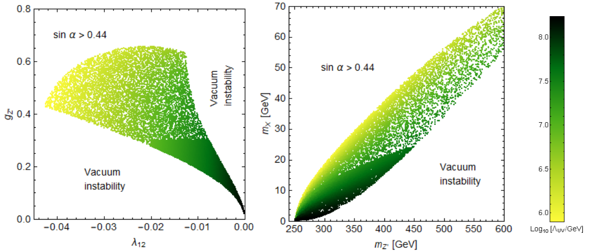
Figure 3: Largest possible UV scales in the QP scenario B of the Hempfling model where the Higgs is the heavier scalar particle.
