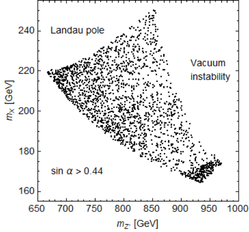
Figure 2: Allowed mass ranges for the new scalar and Z' particles in the Quantum Potential scenario A ( m_X > m_h ) which are perturbatively stable up to the Planck scale. The scenario B ( m_X < m_h ) always breaks down before reaching the Planck scale.
