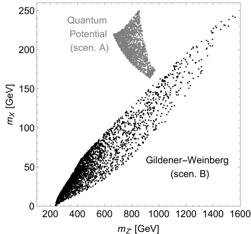
Figure 7: Comparison of Gildener–Weinberg (GW) and Quantum Potential (QP) approaches for the masses of the new scalar and Z' boson in the Hempfling model. Only data points with a UV-cutoff at the Planck scale are plotted. Obviously there is no overlap.
