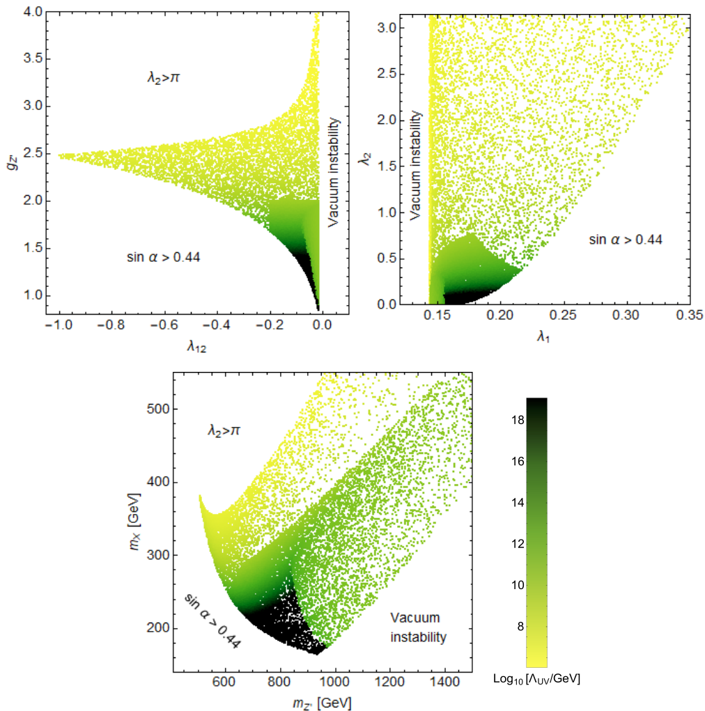
Figure 1: Largest possible UV scales in the QP scenario A of the Hempfling model where the Higgs is the lighter scalar particle.
