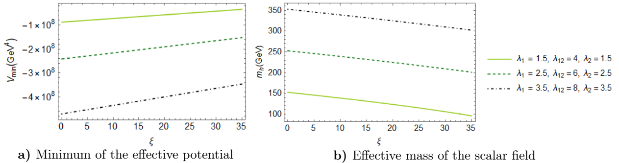
Figure 6: Dependence of the minimum value of the effective potential and effective Higgs mass on the gauge parameter \xi_B = \xi_W = \xi_{Z'} = \xi in the standard model extended by a single scalar field without enforcing a certain hierarchy of couplings.
