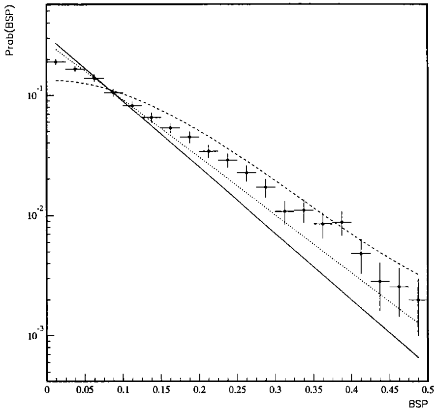
Figure 3: Prob(BSP) distribution for the enriched b sample, for \beta = 0.96 . The lines superimposed correspond to the predictions of JETSET PS for a b\bar{b} branching fraction of 1.0 (dashed line), 0.217 (dotted line), 0. (solid line).
