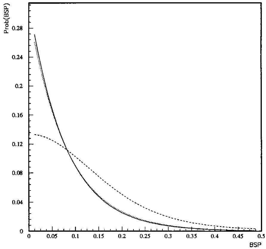
Figure 1: Simulated S_1 \cdot S_2 distribution using JETSET PS for b (dashed line) c (dotted line) and light quarks events (solid line), \beta = 0.96 . The ordinate is the probability per event per bin of 0.025 in the BSP variable ( \equiv \text{Prob}(\text{BSP}) )
