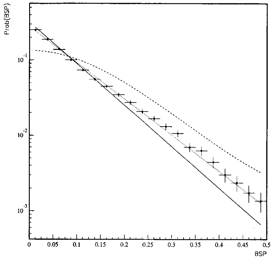
Figure 2: Prob(BSP) distribution, for \beta = 0.96 . The lines superimposed correspond to the predictions of JETSET PS for a Z^0 \rightarrow b\bar{b} branching fraction of 1.0 (dashed line), 0.217, the Standard Model prediction (dotted line), 0.0 (solid line).
