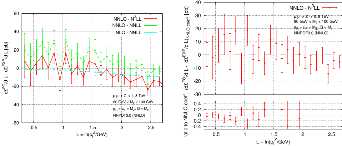
Figure 4. Left: difference between the full NLO and NNLO p_t^Z distribution and the expansion of the NNLL and N^3\text{LL} resummation formulae (3.3) to the respective perturbative order. Right: difference between the fixed-order NNLO coefficient, i.e. the \mathcal{O}(\alpha_s^3) term alone, and the corresponding coefficient from the expansion of the N^3\text{LL} resummation.
