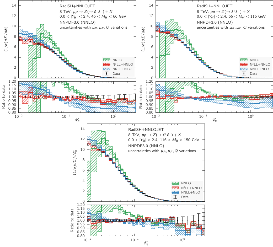
Figure 12. Comparison of the normalised \phi_\eta^* distribution for Drell-Yan pair production at NNLO (green), NNLL+NLO (blue) and N^3LL+NNLO (red) at \sqrt{s} = 8 TeV integrated over the full lepton-pair rapidity range ( 0 < |Y_{\ell\ell}| < 2.4 ), in three different lepton-pair invariant-mass windows. For reference, the ATLAS data is also shown, and the lower panel shows the ratio of each prediction to data.
