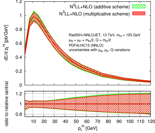
Figure 3. Comparison between additive and multiplicative matching schemes at N^3\text{LL}+\text{NLO} for the transverse momentum distribution for Higgs boson production at \sqrt{s} = 13 \text{ TeV} . The lower panel shows the relative uncertainty bands obtained within the two schemes.
