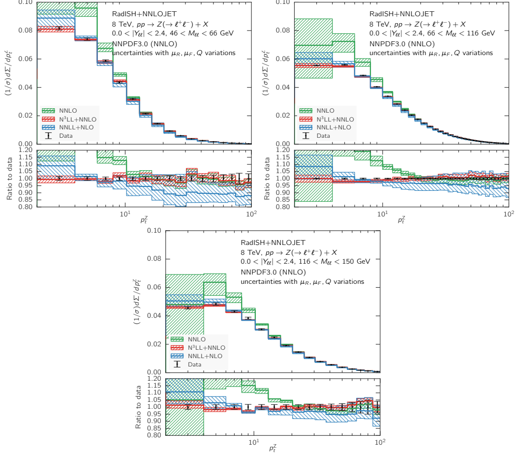
Figure 10. Comparison of the normalised transverse momentum distribution for Drell-Yan pair production at NNLO (green), NNLL+NLO (blue) and N^3\text{LL}+\text{NNLO} (red) at \sqrt{s} = 8 TeV integrated over the full lepton-pair rapidity range ( 0 < |Y_{\ell\ell}| < 2.4 ), in three different lepton-pair invariant-mass windows. For reference, the ATLAS data is also shown, and the lower panel shows the ratio of each prediction to data.
