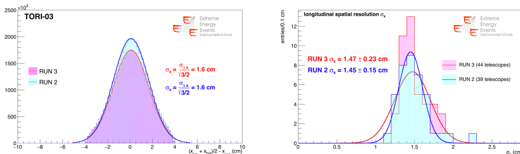
Figure 11. Left: example of longitudinal spatial resolution for one EEE telescope (TORI-03, located in Piedmont) in Run 2 and Run 3, obtained from a subsample of the data used for the whole analysis. Right: longitudinal spatial resolution measured with data taken in Run 2 (Run 3) for n = 39 (44) telescopes of the EEE network.
