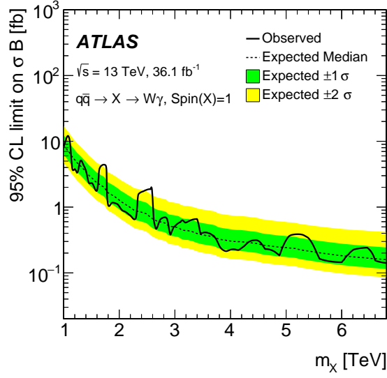
Figure 9: The 95% CL observed (solid line) and expected (dashed line) upper limits on \sigma B for a spin-1 resonance decaying to W\gamma as a function of the resonance mass. The inner and outer bands give the \pm 1 and \pm 2 standard deviations of expected limits. The local deviations of the observed upper limits from the expected ones on \sigma B are a result of small deviations in the data from the best-fitting background-only model.
