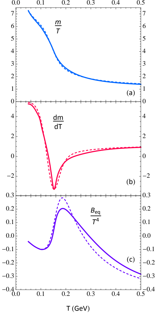
FIG. 1. (Color online) The normalized quasiparticle mass z = m/T (a), the derivative dm/dT (b) and the equilibrium mean field B_{\text{eq}}/T^4 (c) obtained from Eqs. (47) and (48) using a state-of-the-art lattice QCD EOS compiled by the BEST Collaboration [68] (solid lines) and from earlier lattice QCD results obtained by the Wuppertal-Budapest Collaboration [62, 64] (dashed lines), shown as functions of temperature T . In practice, the equilibrium mean field in panel (c) is obtained as the difference between the equilibrium kinetic and lattice QCD pressures, B_{\text{eq}} = \mathcal{P}_{\text{eq}}^{(k)} - \mathcal{P}_{\text{eq}}^{(q)} = \mathcal{P}_{\text{eq}}^{(k)} - \mathcal{P}_{\text{eq}} (see Eq. (45)).
