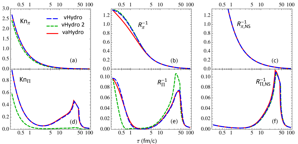
FIG. 6. (Color online) The shear and bulk Knudsen numbers and inverse Reynolds numbers associated with Fig. 5.
