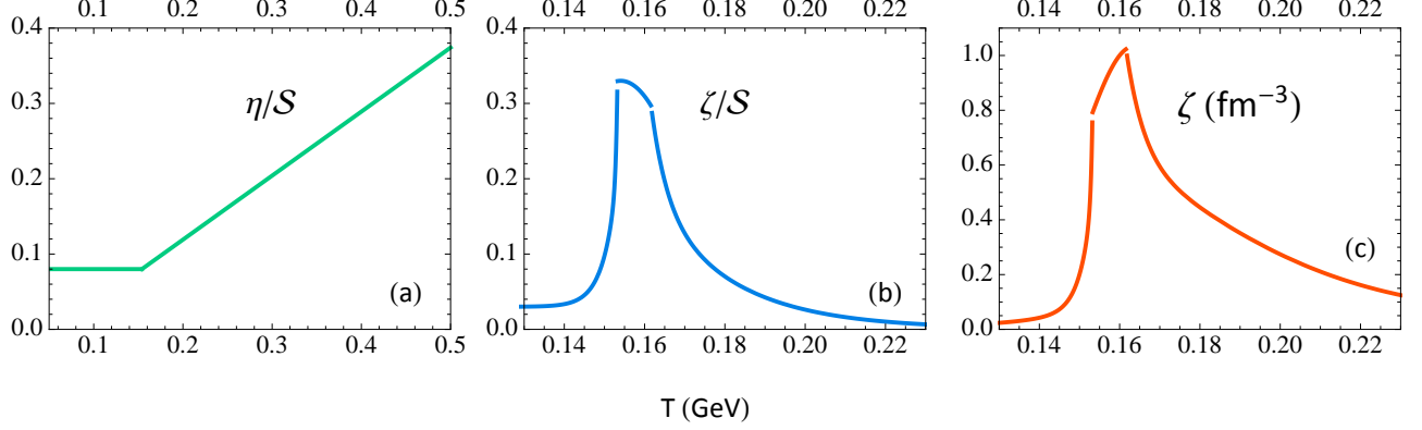
FIG. 2. (Color online) The temperature dependence of (a) the specific shear viscosity \eta/S , (b) the specific bulk viscosity \zeta/S , and (c) the bulk viscosity \zeta itself in units of \text{fm}^{-3} , given by the parameterizations (78) and (79) [6]. We note that the peak of \zeta/S in (b) occurs at the temperature T = 0.995 T_c \approx T_c whereas the bulk viscosity \zeta = (\zeta/S) \times S in panel (c) peaks at the higher temperature T = 1.05 T_c .
