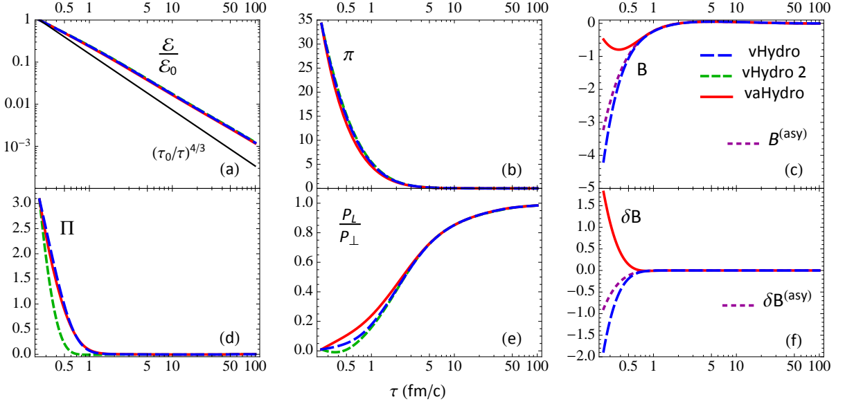
FIG. 5. (Color online) Same as Fig. 3 but for Glasma-like initial conditions, with the same initial temperature at the same initial time. The initial pressures are set to \mathcal{P}_{L0} = 4.975 \times 10^{-3} \mathcal{E}_0 and \mathcal{P}_{\perp 0} = 0.4975 \mathcal{E}_0 . For the anisotropic hydrodynamic evolution (solid red line) the magnitude of the initial mean field B_0 is reduced to 15.3% of the default value (purple short-dashed line) B^{(\text{asy})} = B_{\text{eq}} + \delta B^{(\text{asy})} . For the standard viscous hydrodynamic evolution with quasiparticle transport coefficients (long-dashed blue lines) B and \delta B are determined as described in the text. \Pi , \pi , B , and \delta B are plotted in units of \text{GeV}/\text{fm}^3 .
