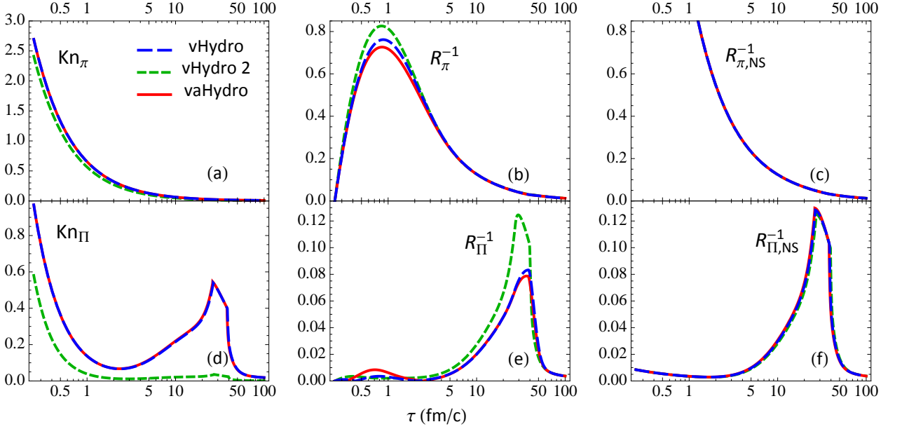
FIG. 4. (Color online) The shear (top row) and bulk (bottom row) Knudsen and inverse Reynolds numbers associated with Fig. 3. For Bjorken flow, the formulas for the Knudsen and inverse Reynolds numbers reduce to \text{Kn}_\pi = \tau_\pi \sqrt{\sigma_{\mu\nu} \sigma^{\mu\nu}} = \sqrt{2/3} \tau_\pi / \tau , \text{Kn}_\Pi = \tau_\Pi \theta = \tau_\Pi / \tau , R_\pi^{-1} = \sqrt{\pi_{\mu\nu} \pi^{\mu\nu}} / \mathcal{P}_{\text{eq}} = \sqrt{3/2} \pi / \mathcal{P}_{\text{eq}} , and R_\Pi^{-1} = |\Pi| / \mathcal{P}_{\text{eq}} . The last column (panels (c,f)) shows the Navier-Stokes limits of the shear and bulk inverse Reynolds numbers, R_{\pi,\text{NS}}^{-1} = \sqrt{8/3} \eta / (\tau \mathcal{P}_{\text{eq}}) and R_{\Pi,\text{NS}}^{-1} = \zeta / (\tau \mathcal{P}_{\text{eq}}) .
