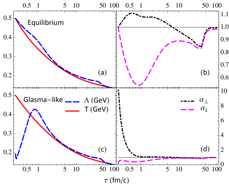
FIG. 7. (Color online) The anisotropic hydrodynamic evolution of the effective temperature \Lambda (dashed blue) compared to the temperature T (solid red) is shown in the left panels for equilibrium (a) and Glasma-like initial conditions (c). The right panels show the evolution of the momentum deformation parameters \alpha_L (dashed magenta) and \alpha_\perp (dash-dotted black), again for equilibrium (b) and Glasma-like initial conditions (d). The temperatures \Lambda and T are plotted in units of GeV. The deformation parameters \alpha_L and \alpha_\perp are unitless.
