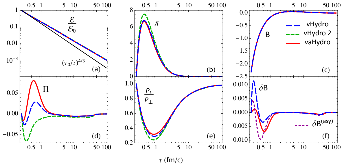
FIG. 3. (Color online) The Bjorken evolution of the normalized energy density \mathcal{E}/\mathcal{E}_0 , bulk viscous pressure \Pi , longitudinal shear stress component \pi , pressure anisotropy \mathcal{P}_L/\mathcal{P}_\perp , total mean field B , and non-equilibrium component of the mean field \delta B , calculated in anisotropic hydrodynamics (solid red, vaHydro) as well as in standard viscous hydrodynamics (dashed blue and green, vHydro and vHydro 2). The solid red and long-dashed blue lines (vaHydro and vHydro) use transport coefficients derived from kinetic theory for medium-dependent quasiparticles while the dashed green lines (vHydro 2) use kinetic theory transport coefficients derived in the small fixed mass limit. The fluid starts out in thermal equilibrium at longitudinal proper time \tau_0 = 0.25 \text{ fm}/c with initial temperature T_0 = 0.5 \text{ GeV} . In panel (f), the short-dashed purple line shows the “asymptotic approximation” (75) for \delta B , computed using data from the anisotropic hydrodynamic evolution whereas the long-dashed blue line uses Eq. (84) and data from the viscous hydrodynamic evolution. \Pi , \pi , B , and \delta B are plotted in units of \text{GeV}/\text{fm}^3 .
