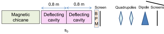
Fig. 2. Schematic of the lattice design at the TDS. Element positions are not yet fixed.
