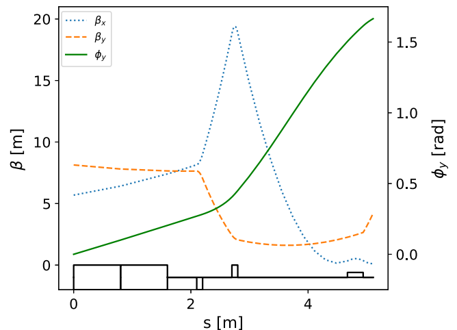
Fig. 3. \beta -functions and vertical phase advance for the lattice design, ending at the screen at s = 5.11 m. The positions of the two TDS cavities, the two quadrupoles and the dipole are indicated at the bottom.
