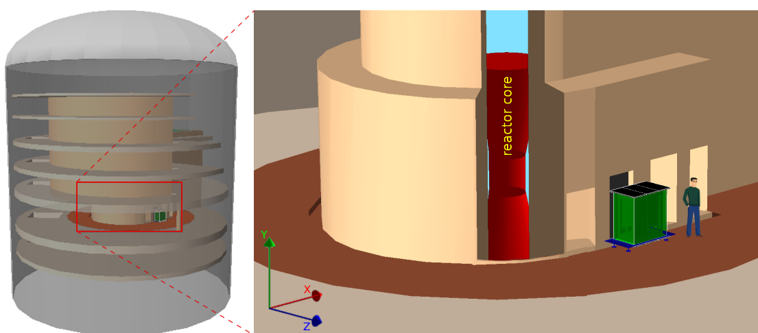
Figure 13. Sketch of the BR2 containment building and the prototype detector simulated in GEANT4.
