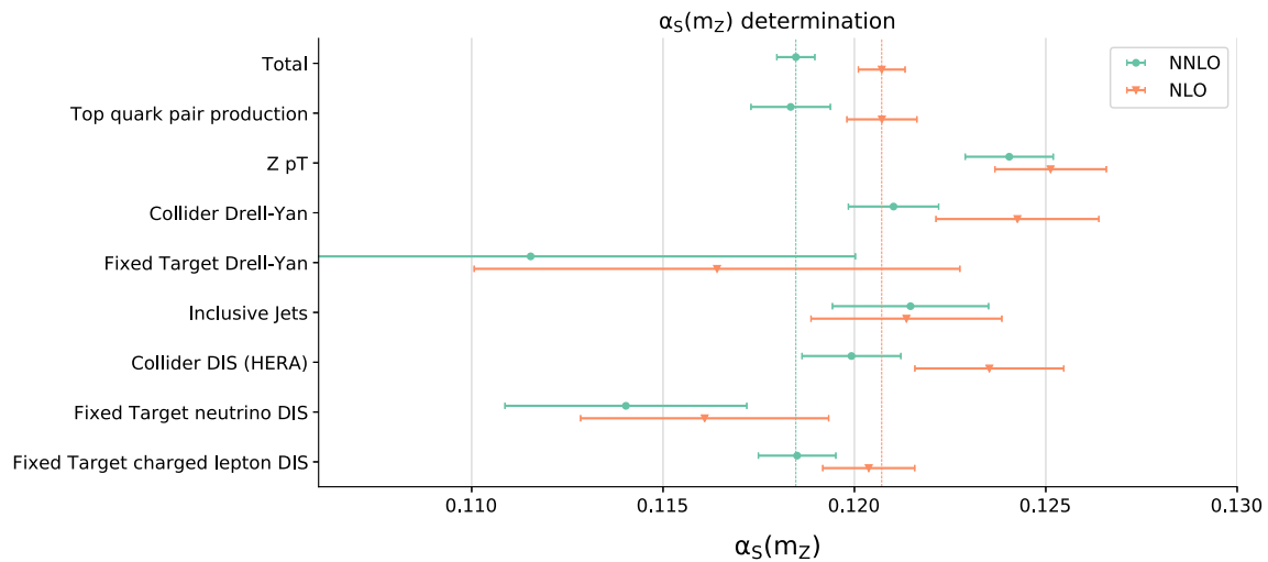
Fig. 4 The values of the partial \alpha_s(m_Z) and the corresponding uncertainties determined from \chi^2_p for the various families of processes p of Table 1 at NLO and NNLO
