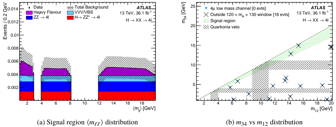
Figure 6: Distribution of (a) \langle m_{\ell\ell} \rangle = \frac{1}{2}(m_{12} + m_{34}) and (b) m_{34} vs m_{12} , for events selected in the H \rightarrow XX \rightarrow 4\mu(1 < m_X < 15 \text{ GeV}) analysis. The crossed-through points in figure (b) correspond to events that are outside the m_{4\ell} mass window of 120 \text{ GeV} < m_{4\ell} < 130 \text{ GeV} . The events outside the (shaded green) signal region are events that fail the m_{34}/m_{12} > 0.85 requirement.
