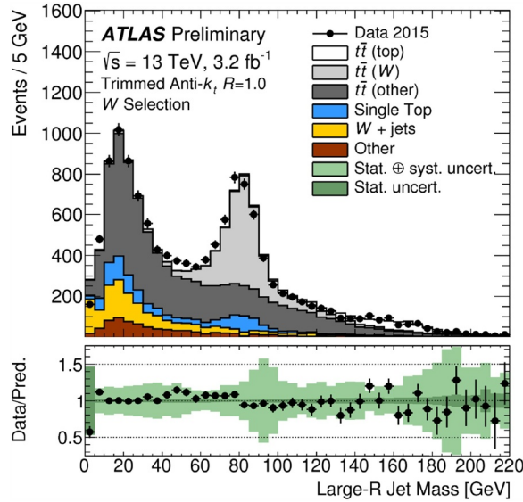
Fig. 9. Distribution of the calorimeter jet mass spectrum for the leading- p_T jet, in the ATLAS experiment, in 13 TeV data and MC simulation using trimmed [108] anti- k_r R=1.0 jets, with trimming parameters f_{\text{cut}} = 5\% and R_{\text{sub}} = 0.2 in lepton + jets events. The large R jets are required to have p_T > 200 GeV [109].
