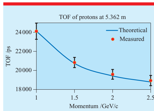
Figure 9. TOF of protons at 5.362 m. The blue line corresponds to the theoretically predicted values and the red dots to the measured ones.
