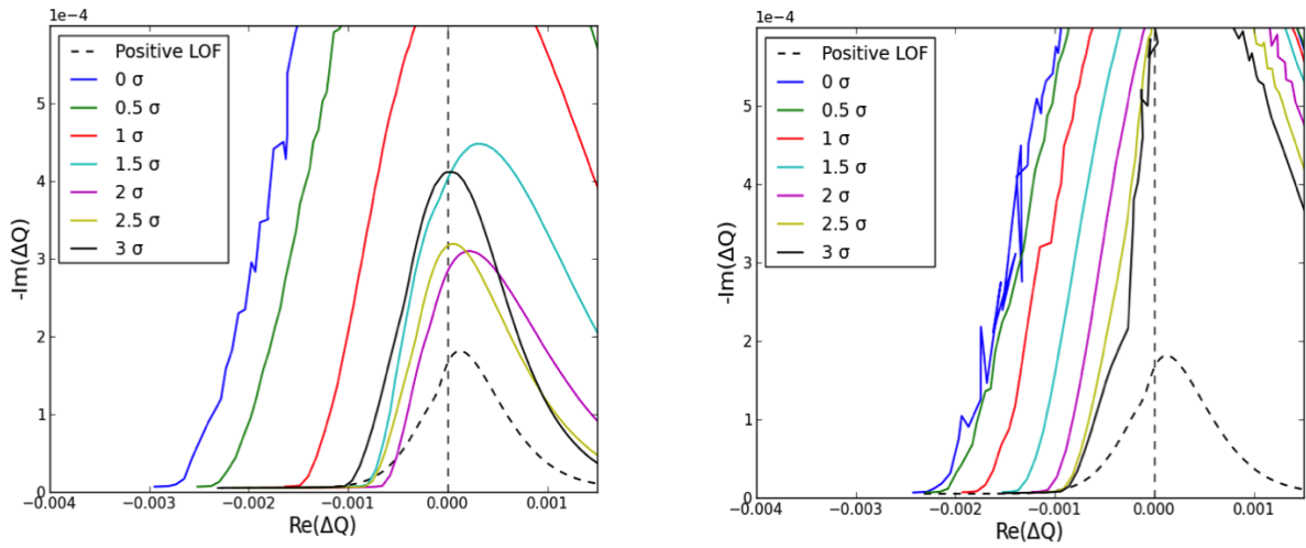
Figure 21: Horizontal (left) and Vertical Stability diagrams computed for a typical physics fill for different transverse separations at IP1 (legend). In dashed black lines the stability diagrams due to octupoles alone are plotted as a reference.
