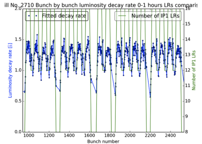
Figure 1: Bunch by bunch luminosity decay rate computed for first hour in stable beams during a representative physics fill number 2710 of the LHC physics fills of 2012.
