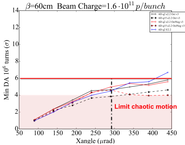
Figure 4: Dynamic aperture calculations as a function of the crossing angle \alpha in IP1 and IP5 for the LHC standard configuration during the 2012 physics run: 60 \beta^* at the two IPs, bunch intensities of 1.6 \times 10^{11} protons and normalized transverse emittances of 2.2 \mu\text{m} . The different lines corresponds to beam-beam alone (blue line), with positive octupole polarity operation (black lines) and negative octupole polarity operation with 550 A current (red lines). The solid lines refer to operation with low chromaticity ( Q' = 2 units) while dashed lines are for high chromaticity operation ( Q' = 15 units). The limit of chaotic motion identified empirically during experiments [6–9] is highlighted as the red area below 4\sigma dynamic aperture.
