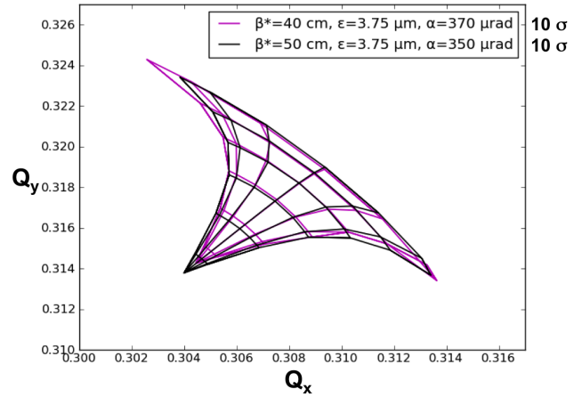
Figure 15: 2 Dimensional detuning with amplitude, footprint, for a separation of 10 \sigma in IP1 and IP5 for two possible optics the 40 (pink line) and 50 cm (black line).
