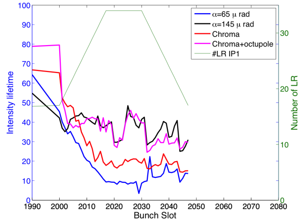
Figure 10: Beam 1 bunch by bunch lifetimes in hours as a function of the bunch slot position for the operational half crossing angle ( \alpha/2 = 145 \mu rad black line), for the reduced angle ( \alpha/2 = 65 \mu rad blue line), reduced chromaticity ( Q' reduced from 15 to 2 units, red line) and for reduced current in the octupole magnets (from 476 A to zero, pink line). The number of long-range encounters as a function of the 25 ns slot number are also shown (green line).
