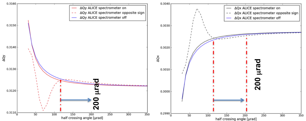
Figure 19: Vertical (left picture) and horizontal (right picture) tune shifted caused by the beam-beam effects at IP2 (the Alice experiment). The solid blue lines refer to the case without the spectrometer, red solid line to the case with spectrometer with polarity that sum up with the long-range beam-beam while the dashed line to the case with polarity that reduces the separation of the beam-beam encounters. The proposed half crossing angle to allow swap of spectrometer polarity is shown and is 200 \mu rad .
