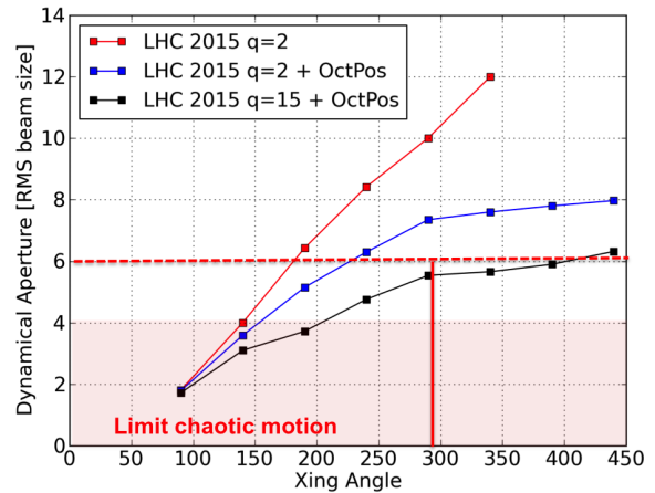
Figure 5: Dynamic aperture calculations as a function of the crossing angle \alpha in IP1 and IP5 for the LHC standard configuration during the 2015 physics run: 80 \beta^* at the two IPs, bunch intensities of 1.3 \times 10^{11} protons and normalized transverse emittances of 3.75 \mu\text{m} . The different lines corresponds to beam-beam alone (red line), with octupoles at 550 A in positive polarity operation (blue lines) and high chromaticity 15 units (black lines). The limit of chaotic motion identified empirically during experiments [6–9] is highlighted as the red area below 4 \sigma dynamic aperture.
