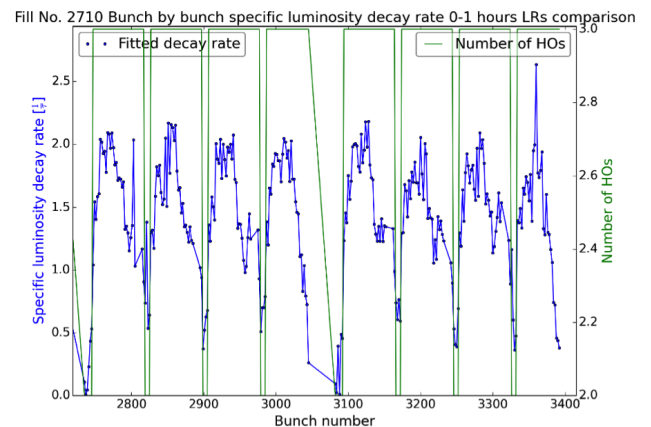
Figure 2: Bunch by bunch specific luminosity decay rate computed for first hour in stable beams during a representative physics fill number 2710 of the LHC physics fills of 2012.
