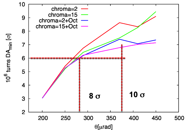
Figure 13: Dynamic aperture calculations for a 4D case (without longitudinal motion) as a function of the crossing angle \alpha in IP1 and IP5 for the 2016 LHC configuration: 40 \beta^* at the two IPs, bunch intensities of 1.3 \times 10^{11} protons and normalised transverse emittances of 3.75 \mu\text{m} . The different lines corresponds to beam-beam head-on and long-range interactions with chromaticity of 2 units (red line), with chromaticity of 15 units (green line), with octupoles at current of 476 A in positive polarity (blue line) and with chromaticity of 15 units and octupole at 476 A (pink line). The proposed crossing angle of 370 \mu\text{rad} corresponding to 10 \sigma beam to beam separation at the first long-range encounter is high lighted with the potential lower limit of 8 \sigma separation.
