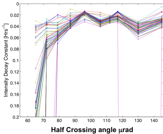
Figure 9: Beam 2 bunch by bunch intensity decay rates as a function of the half crossing angle \alpha/2 at IP1 and IP5.
