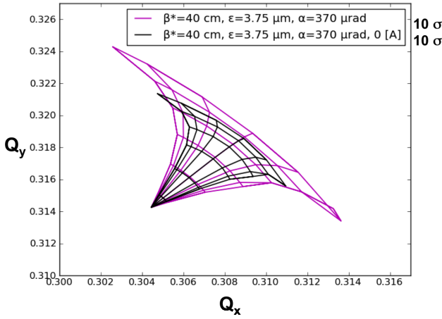
Figure 17: 2 Dimensional detuning with amplitude, footprint, for the 2016 physics run with (pink line) and without (black line) octupole magnets detuning.
