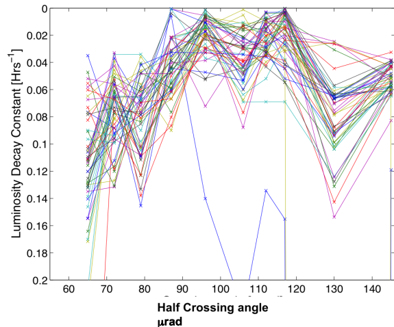
Figure 11: Bunch by bunch luminosity decay rate as a function of the half crossing angle \alpha/2 at IP1 and IP5.
