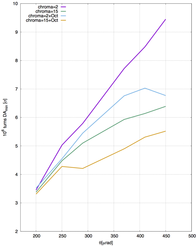
Figure 14: 6 D Dynamic aperture calculations as a function of the crossing angle \alpha in IP1 and IP5 for the 2016 LHC configuration: 40 \beta^* at the two IPs, bunch intensities of 1.3 \times 10^{11} protons and normalised transverse emittances of 3.75 \mu\text{m} . The different lines corresponds to beam-beam head-on and long-range interactions with chromaticity of 2 units (red line), with chromaticity of 15 units (green line), with octupoles at current of 476 A in positive polarity (blue line) and with chromaticity of 15 units and octupole at 476 A (pink line). The proposed crossing angle of 370 \mu\text{rad} corresponding to 10 \sigma beam to beam separation at the first long-range encounter is high lighted with the potential lower limit of 8 \sigma separation.
