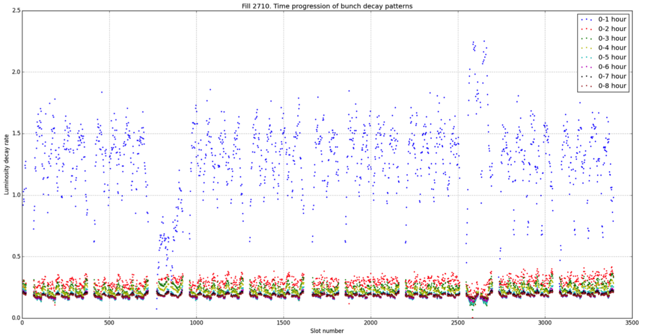
Figure 3: Bunch by bunch luminosity decay rates for different time intervals (see legend) for the LHC physics fill number 2710 of 8 hours in stable beams. The decay rates are computed using different time intervals to show the impact of long range beam-beam effect (blue dots pattern) dominant in the first hour of physics fill and disappearing after (red, green dots as expressed in the legend).
