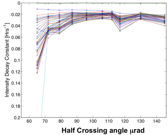
Figure 8: Beam 1 bunch by bunch intensity decay rates as a function of the half crossing angle \alpha/2 at IP1 and IP5.
