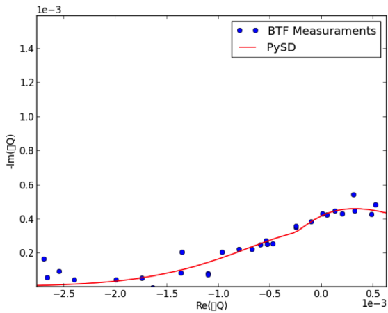
Figure 22: Computed (red line ) versus measured (BTF reconstruction) stability diagram.
