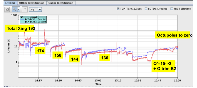
Figure 7: Beam 1 (blue line) and beam 2 (red line) loss lifetimes in hours as a function of time during the long-range test done on 15th September 2015 in the LHC. In yellow the steps can find the reduced crossing angles at IP1 and IP5 during the MD. The reduction of chromaticity from 15 to 2 units and octupole magnet current from 476 A to zero are also highlighted as last two steps of the experiment.
