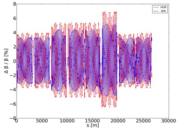
Figure 23: Horizontal (red) and Vertical (blue) beta-beating percentage due to beam-beam effects for a typical 2015 physics fill along the LHC circumference starting from IP3.
