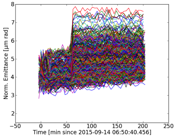
Figure 20: Bunch by bunch emittances in \mu\text{m} as a function of time during a physics fill of 2015 physics run. The emittances are measured by the BSRTs showing a sudden increase on selected bunches while beams were separated.
