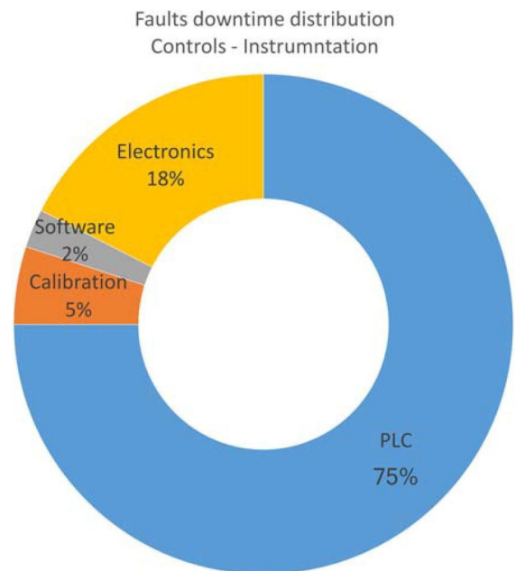
Figure 8: Breakdown of controls and communication faults
