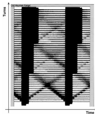
Figure 11.23: COLDEX MD2: 1% of the beam is uncaptured at the first batch injection and leads/lags in the longitudinal phase space, as measured by the SPS Mountain Range 200 MHz RF pick-up.
