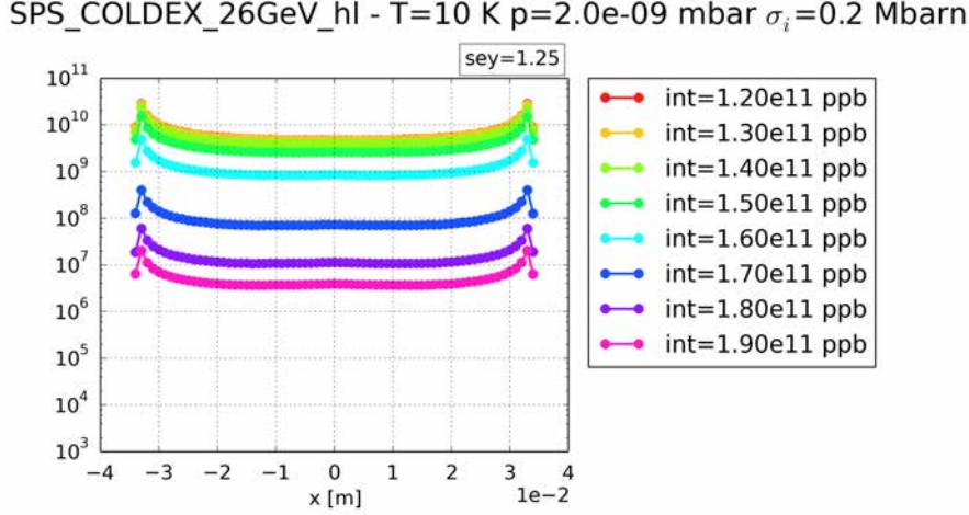
Figure 10.8: Impinging electron flux per vertical slice for SEY=1.25 and different bunch intensities. PyECLOUD simulation, 26 GeV, T=10 K, \sigma_i=0.2 Mbarn.
