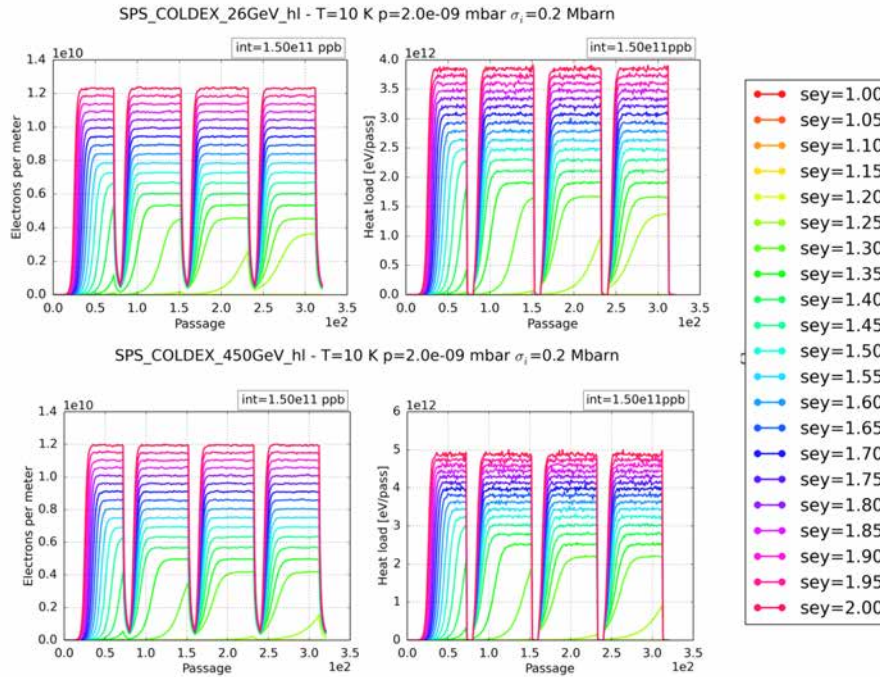
Figure 10.11: Electron density per passage (left) and sum of the kinetic energies of the impinging electrons (right) vs SEY for 1.5 \cdot 10^{11} ppb. PyELOUD simulation, 26 GeV (top) and 450 GeV (bottom), T=10 K, \sigma_i=0.2 Mbarn.
