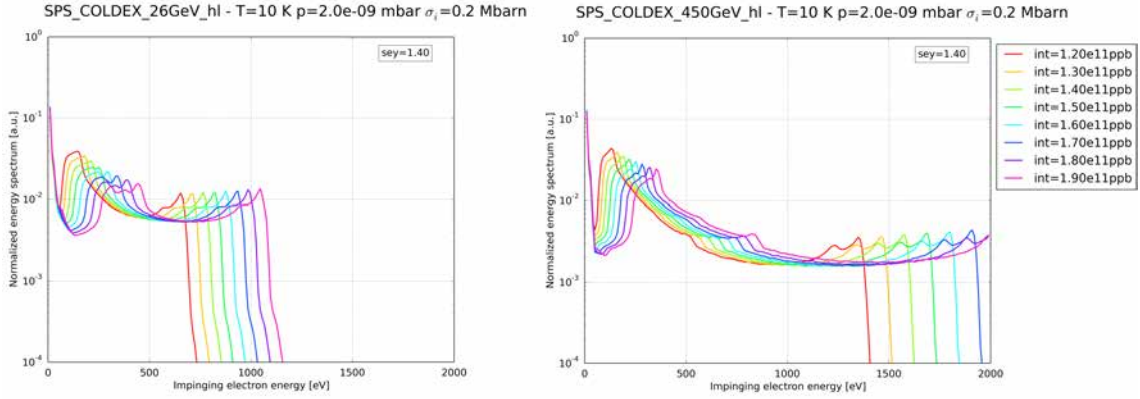
Figure 10.10: Normalized impinging electrons energy spectra (over 320 passages) in the case of SEY=1.4, for different bunch intensities. PyELOUD simulation, 26 GeV (left) and 450 GeV (right), T=10 K, \sigma_i=0.2 Mbarn.
