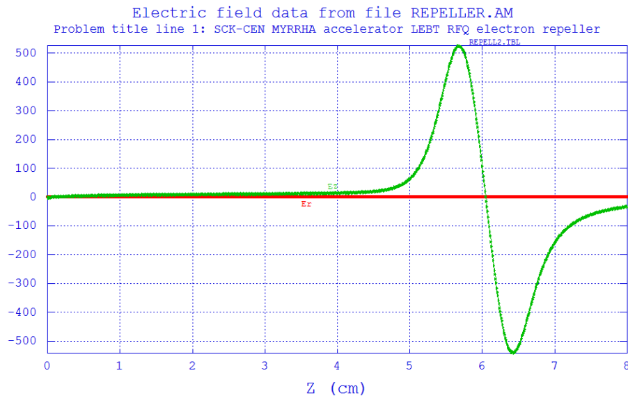
Figure 6.34: Longitudinal E_z (green) and radial E_r (red) electric field components, along the z axis in the longitudinal rz plane, of MYRRHA LEPT RFQ collimator electron repeller.
