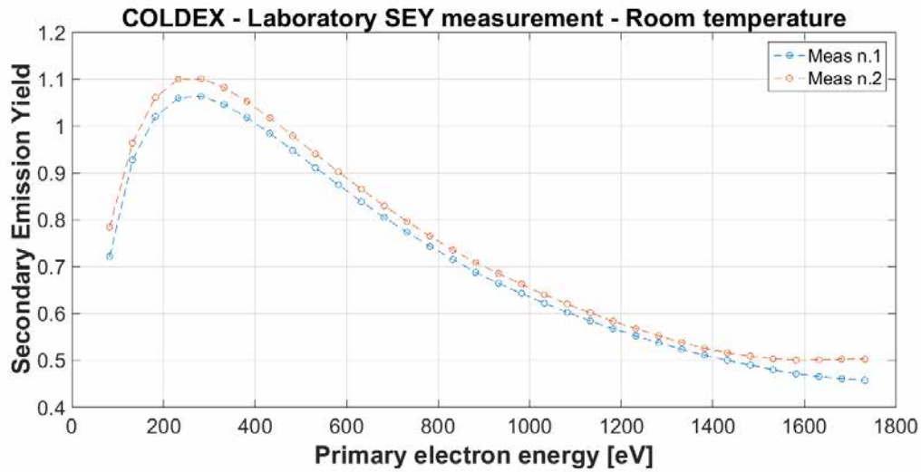
Figure 9.1: Laboratory measurements of SEY on one witness sample obtained during COLDEX BS a-C coating.
