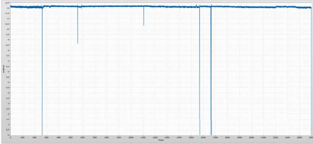
Figure 6.41: Snapshot of the recorded H^+ beam intensity during the MYRRHA Ion Source FATs. The vertical peaks correspond to instabilities in the beam intensity mainly caused by HV sparking.
