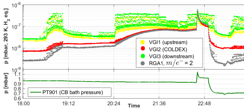
Figure 11.12: COLDEX Run 3: zoom after the BS warm-up to 60K, showing the monolayer build-up of the CB caused by transmission of the gas desorbed at the RT extremities due to electron cloud.
