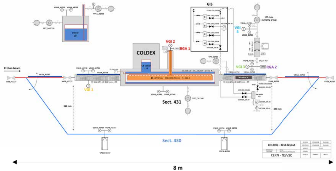
Figure 9.11: Schematic view of SPS/LSS4 vacuum sectors 430 and 431 vacuum devices and instrumentation following 2014 COLDEX recommissioning and further 2016 upgrade (new GIS).
