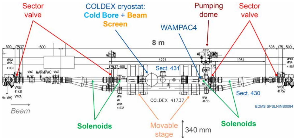
Figure 9.2: Layout of sectors 431/430 elaborated from the SPS LSS4 layout drawing of period 41410-42210 (SPSLNINS0084).
