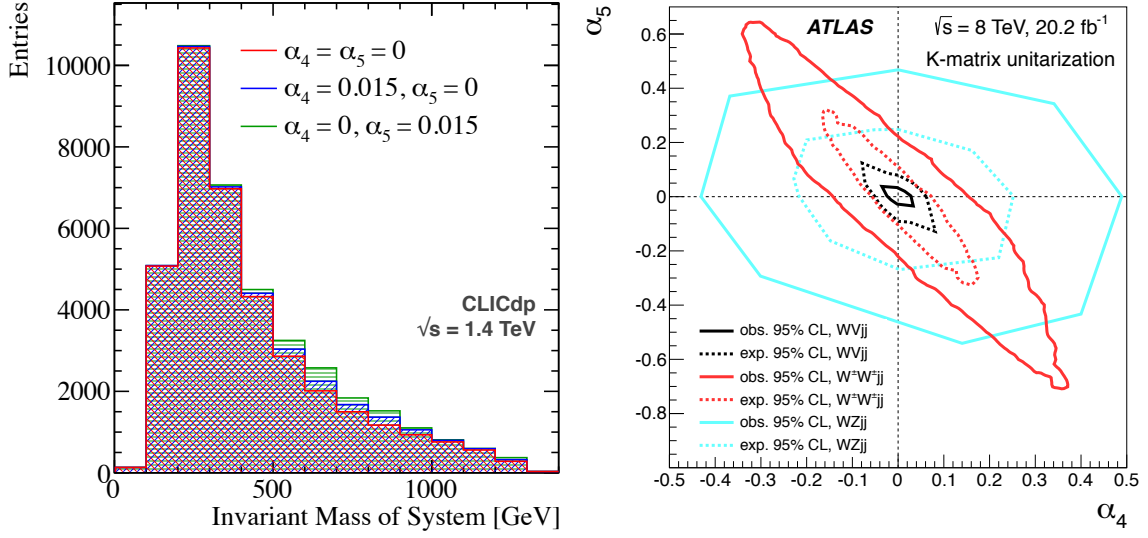
Figure 1: The invariant mass of the four jet system for different values of \alpha_4 and \alpha_5 for CLIC running at 1.4 TeV (left) and limits on anomalous electroweak production of WW and WZ by ATLAS using the full 8 TeV LHC Run I data of 20.2 \text{ fb}^{-1} [10] (right).
