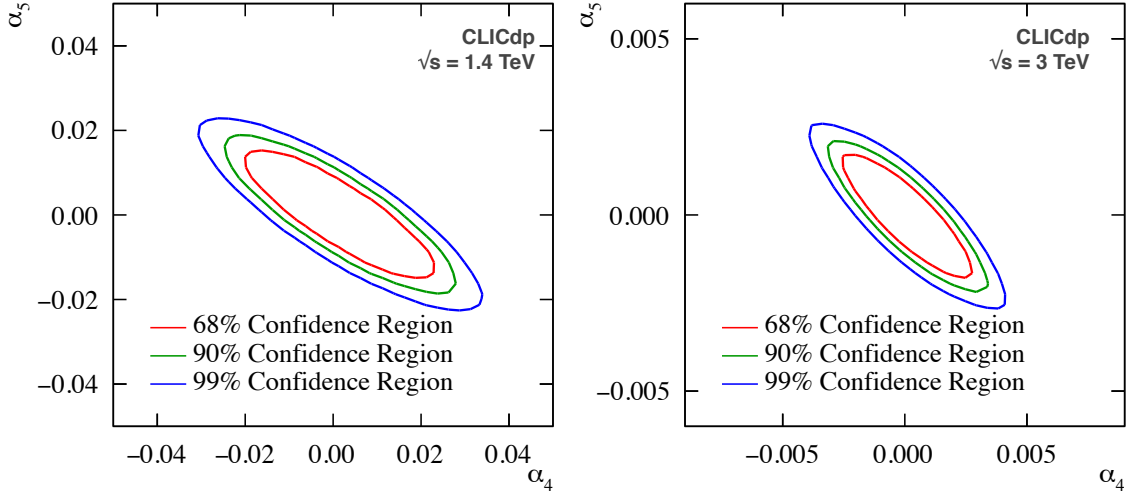
Figure 2: Projected sensitivity to \alpha_4 and \alpha_5 for CLIC after completion of the 1.4 TeV run with 1.5 \text{ ab}^{-1} integrated luminosity (left) and using a 3 TeV dataset of 2 \text{ ab}^{-1} .
