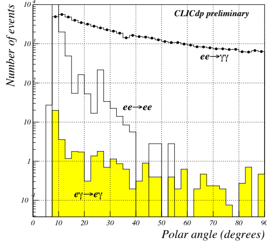
Figure 3: Signal and background contributions to the reconstructed di-photon spectrum at CLIC as function of the photon polar angle for an integrated luminosity of 2 \text{ ab}^{-1} at 3 TeV. The photon in the e\gamma \rightarrow e\gamma background (yellow) is picked up from beamstrahlung or quasi-real photons emitted from the incoming electron.
