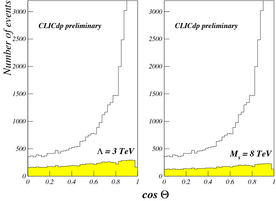
Figure 4: The expected number of signal events for a QED cut-off model with \Lambda_{\text{QED}} = 3 \text{ TeV} (left) and extra dimensions with M_s = 8 \text{ TeV} (right) together with the expected number of events from SM di-photon production as function of \cos\theta for an integrated luminosity of L = 2 \text{ ab}^{-1} at \sqrt{s} = 3 \text{ TeV} .
