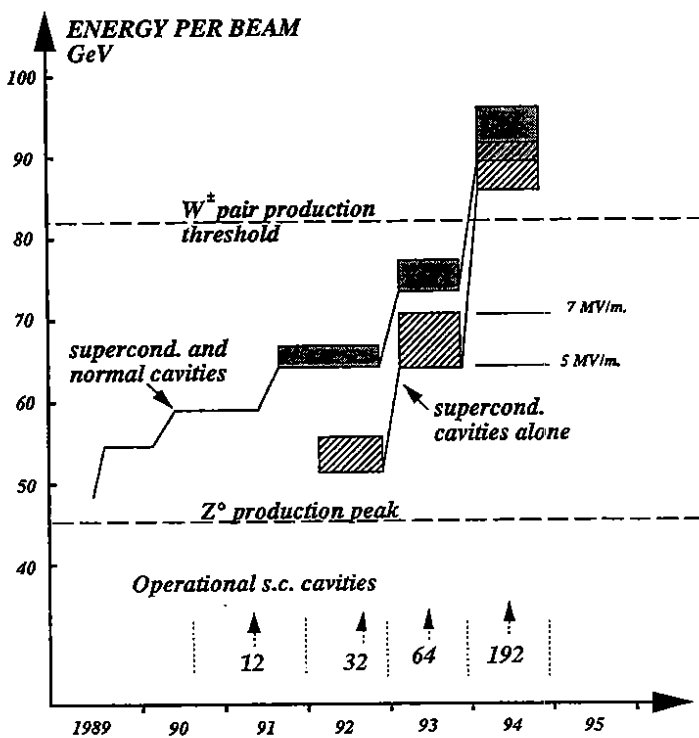
Figure 1. The planned LEP upgrading
