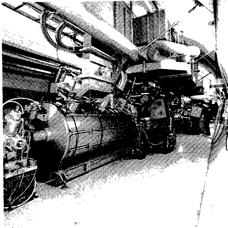
Figure 3. The first module installed in LEP
