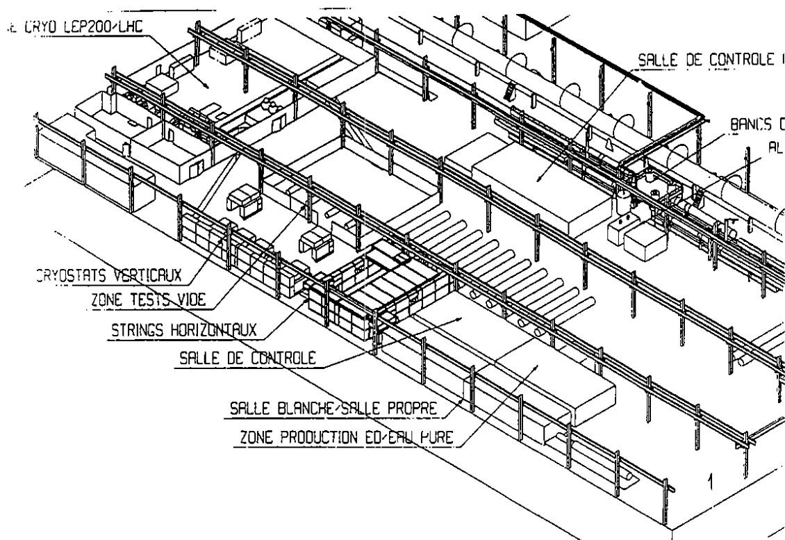
Figure 5. Sketch of the test area under construction
