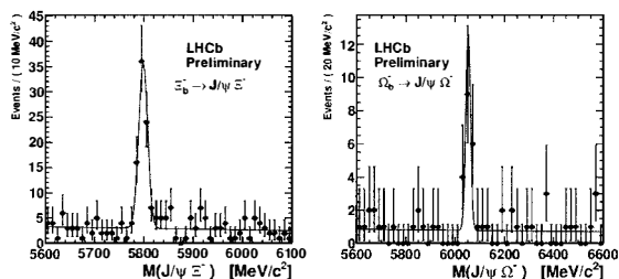
Figure 3: Invariant mass distribution of \Xi_b and \Omega_b with the fit projections overlaid.
