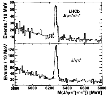
Figure 1: Invariant mass distributions of B_c^+ \rightarrow J/\psi\pi^+\pi^-\pi^+ and B_c^+ \rightarrow J/\psi\pi^+ candidates with the fit overlaid.
