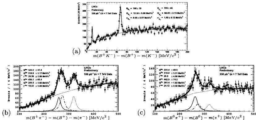
Figure 2: Fits to the Q distributions of the (a) B^+K^- , (b) B^+\pi^- and (c) B^0\pi^+ final states. The full histogram (a) shows the distribution of wrong sign combinations.
