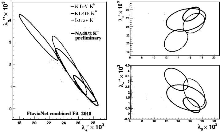
Figure 2: Combined quadratic fit results for K_{13} decays. The ellipses are 68% confidence level contours. For comparison, the combined fit from the FlaviaNet kaon working group is shown 1 .
