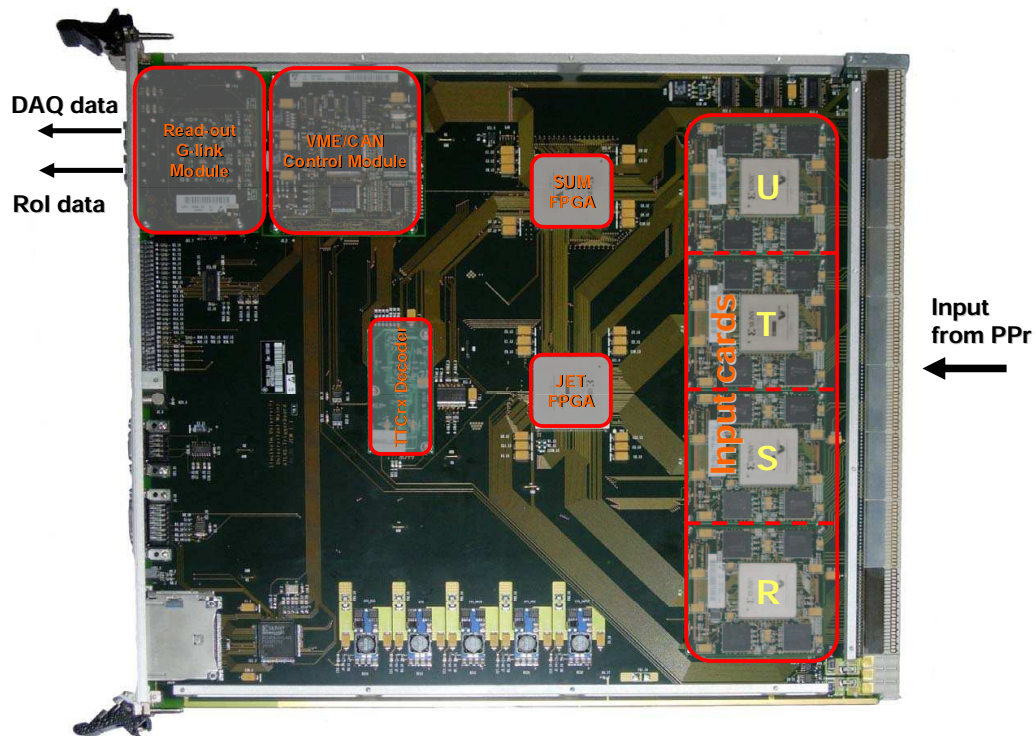
Figure 3.10: JET/Energy-sum Module.
