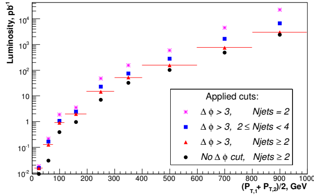
Figure 7.21: Integrated luminosity required to reach 0.5% precision as a function of p_T in the probe region 0.7 < \eta < 0.8 with different sets of cuts: all dijet events (black circles), \Delta\phi > 3 between the two leading jets (red triangles), in addition to \Delta\phi cut, less than 4 jets in an event (blue squares), exactly two reconstructed jets (magenta stars). The reference region is 0 < |\eta| < 0.7 .
