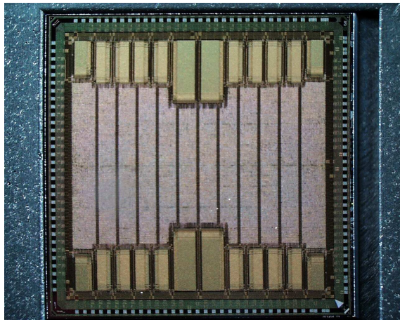
Figure 4.2: The Pre-Processor ASIC die.
