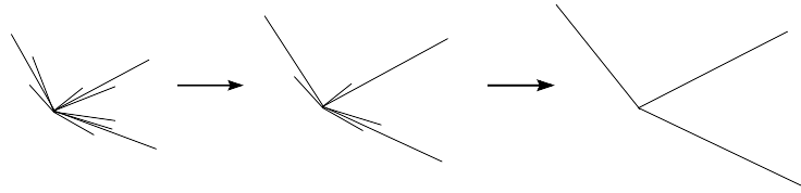
Figure 1.8: A simplified example of the successive iterations of the K_T algorithm.
