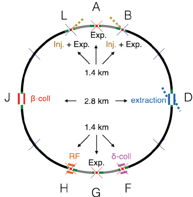
Figure 1: FCC layout [2]. The main EIR are located at A & G, and the low luminosity ones at L & B.
