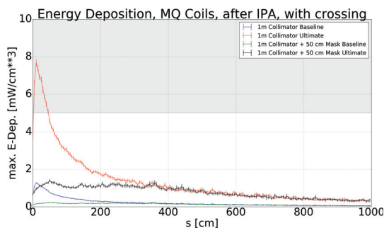
Figure 6: Maximum energy deposition per \text{cm}^3 in 5 cm bins along the first quadrupole in cell 8 after IPA for baseline and ultimate configuration.
