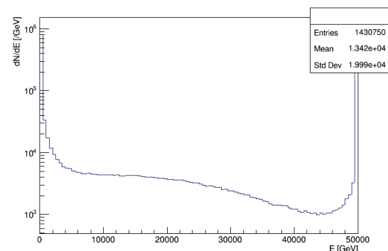
Figure 2: Proton energy distribution 3 m downstream of IPA for 10^6 pp collision events.
