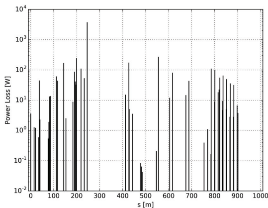
Figure 4: Inelastic proton power loss map per element.
