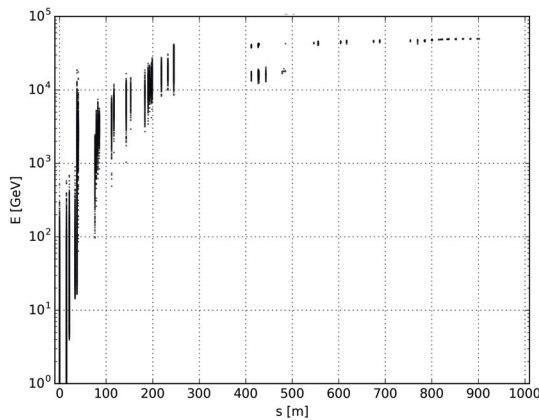
Figure 3: Inelastic proton energy correlation loss map per element. The TAS is located at 40 m, D1 at 230 m, D2 at 425 m, the dispersion suppressor region begins around 800 m, and s = 0 is IPA.
