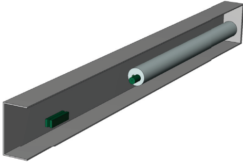
Figure 5: 3D FLUKA model used for shower simulations in the dispersion suppressor. The green objects are first the TCLD collimator, followed by a 50 cm long mask, both made of Inermet180. Following this is the first quadrupole in the DS. The particles are loaded 63 cm before the collimator.
