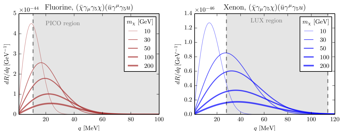
Figure 1. The momentum exchange distributions for DM scattering on a representative light nucleus, ^{19}\text{F} , (left) and heavy nucleus, \text{Xe} , (right) for spin-dependent scattering. The Wilson coefficient of the operator is set to (1 \text{ TeV})^{-2} in both cases and we summed the contributions of the xenon isotopes weighted by their natural abundances. The curves of different thicknesses correspond to different dark matter masses in GeV as shown in the plot legends. The approximate experimental thresholds are denoted by dashed vertical lines. For fluorine, we use the PICO threshold region E_R > 3.3 \text{ keV} [28] while for LUX, we use the approximate region E_R \in [3, 50] \text{ keV} [29].
