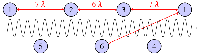
Figure 17. When the recirculation is in place, the linacs are populated with bunches at different turns (the turn number is indicated). The recombination pattern shown maximises separation inside the RF structure between the low energy bunches (at the first and sixth turn).
