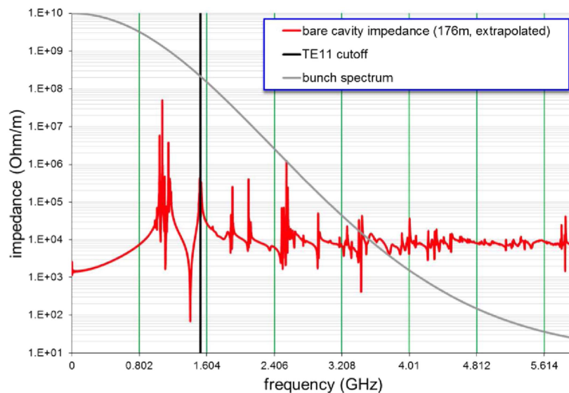
Figure 36. Dipole HOM spectrum of the bare cavity. All harmful modes are well separated from RF harmonics. Impedances of modes below cut-off are unresolved and will be determined by the HOM damping configuration.
