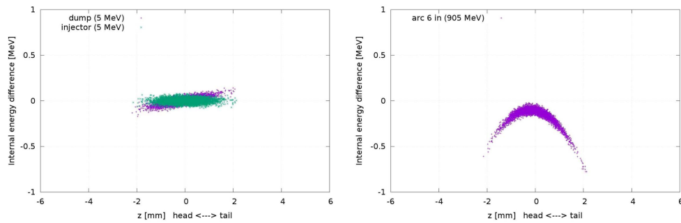
Figure 20. Longitudinal phase space at injector/dump (left) and at 900 MeV (right).
