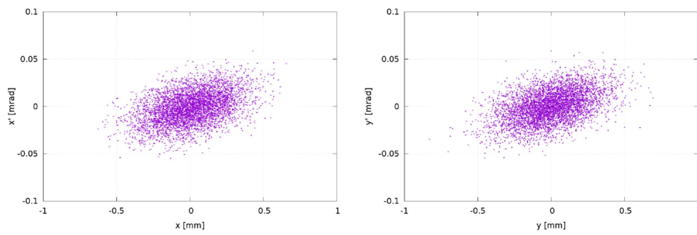
Figure 19. Horizontal and vertical phase space at 900 MeV.
