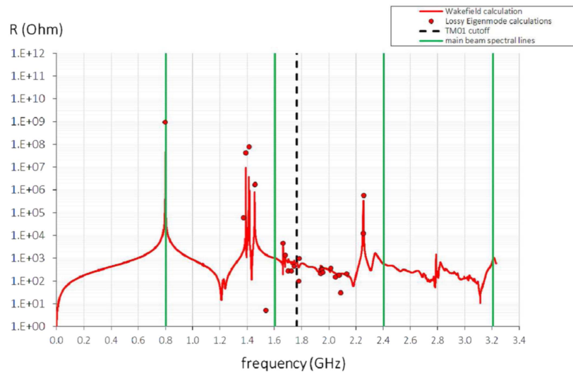
Figure 31. Impedance spectrum for the longitudinal modes as a function of frequency of the low-loss cavity design with iris diameter of 130 mm (compare figure 26).
