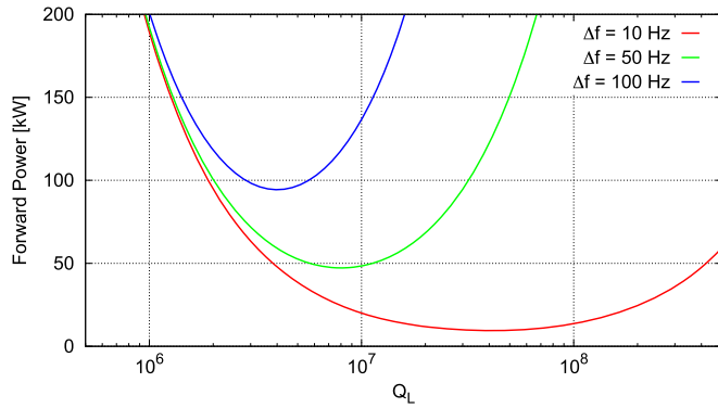
Figure 29. Forward power as a function of the loaded Q , for Q_L \simeq Q_{ext} , of the cavity for different detunings and zero beam loading.
