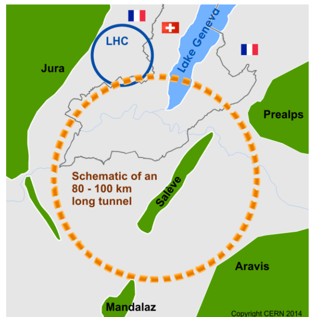
Figure 1: Schematic of a 100 km tunnel for a highest-energy circular collider in the Lake Geneva basin.
