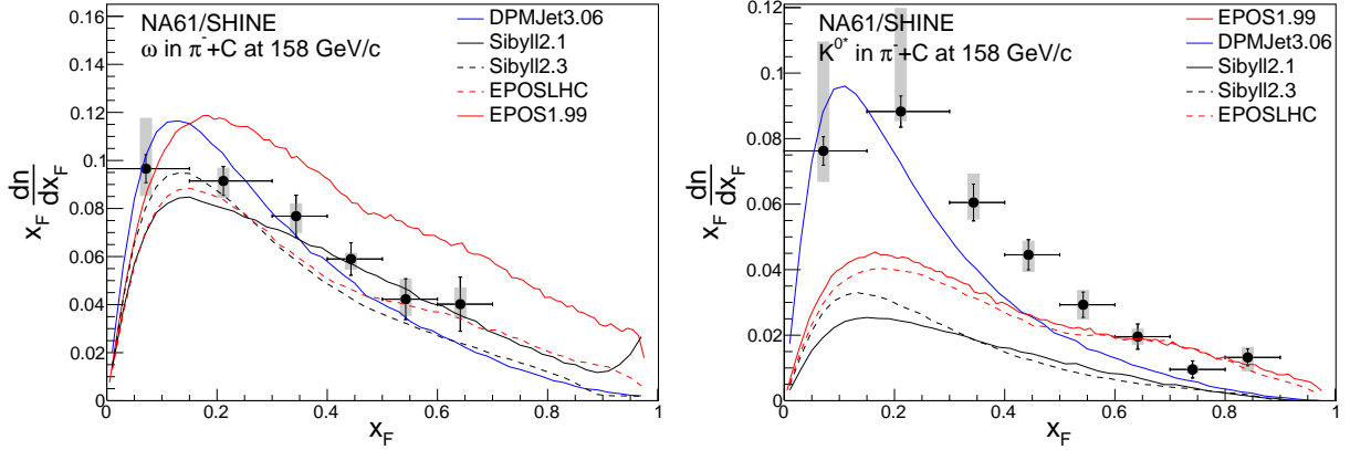
Figure 13: Scaled x_F -spectra of \omega ( left ) and K^{*0} ( right ) mesons, x_F \frac{dn}{dx_F} , in \pi^-+C production interactions at 158 GeV/c. The error bars show the statistical, the bands indicate systematic uncertainties. The lines depict predictions of hadronic interaction models: red – EPOS 1.99, blue – DPMJET 3.06, black – SIBYLL 2.1, dashed red – EPOS LHC, dashed black – SIBYLL 2.3.
