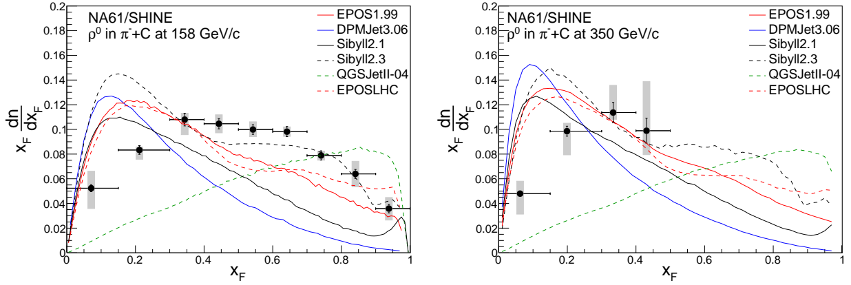
Figure 12: Scaled x_F -spectra of \rho^0 mesons, x_F \frac{dn}{dx_F} , in \pi^-+C production interactions at 158 ( left ) and 350 GeV/c ( right ). The error bars show the statistical, the bands indicate systematic uncertainties. The lines depict predictions of hadronic interaction models: red – EPOS 1.99, blue – DPMJET 3.06, black – SIBYLL 2.1, dashed green – QGSJET II-04, dashed red – EPOS LHC, dashed black – SIBYLL 2.3.
