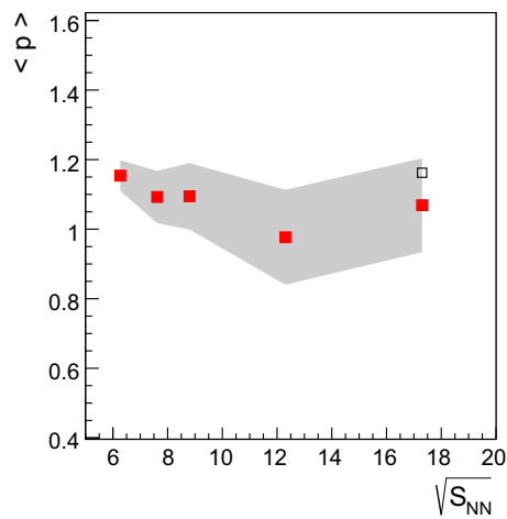
Fig. 38 Mean proton multiplicities produced in inelastic p + p interactions as a function of collision energy. Filled red squares depict results from this analysis, the open black square shows the measurement of NA49 [12]. The dominating uncertainty of the NA61/SHINE measurements is systematic and is indicated by the shaded band
