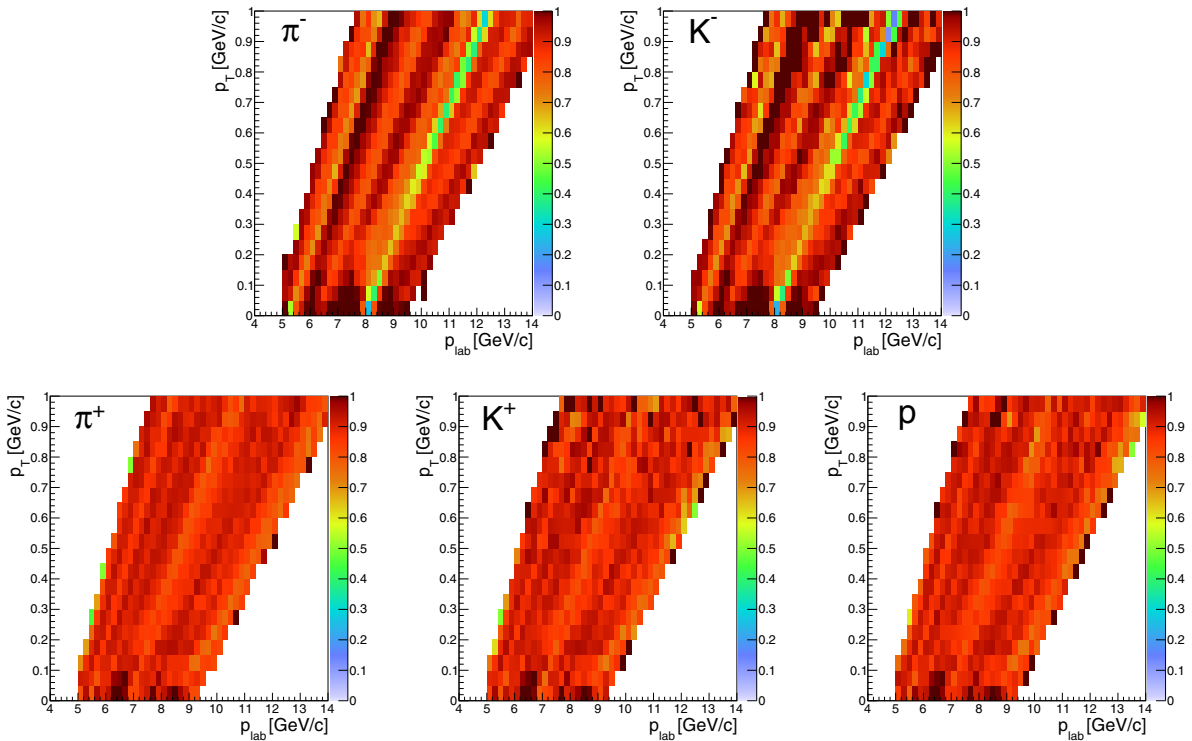
Fig. 47 Fraction of pixels providing a valid ToF measurement for p + p interactions at 158 GeV/c. Visible strips with lower value are due to groups of not working pixels
