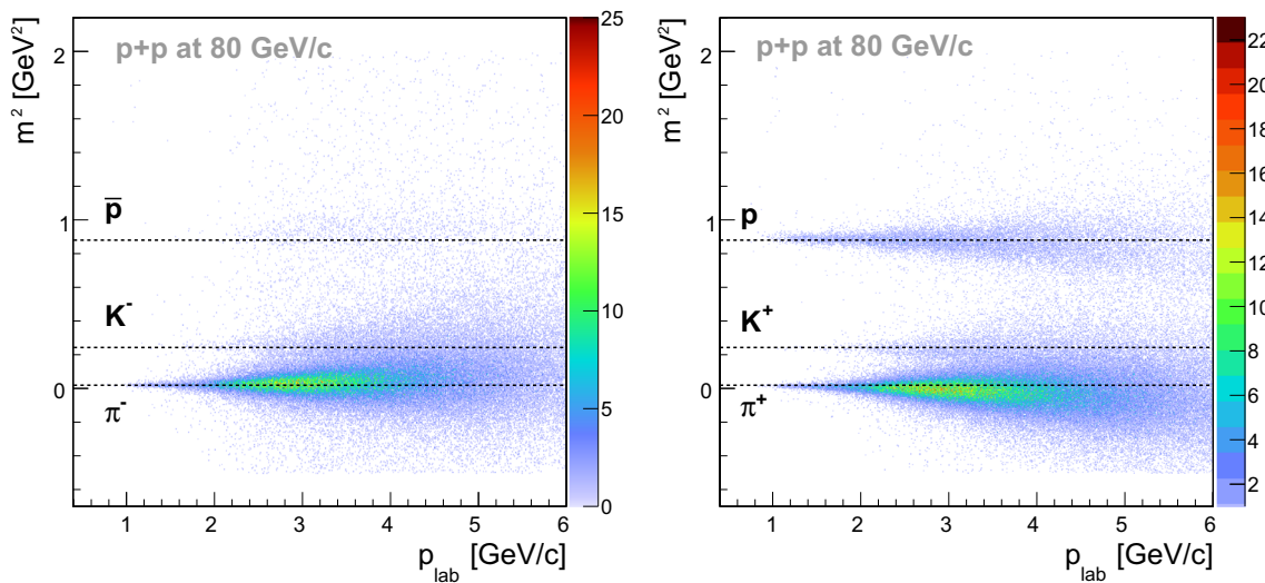
Fig. 7 Mass squared versus momentum measured by ToF-R ( left ) and ToF-L ( right ) detectors for particles produced in p + p interactions at 80 GeV/c. The lines show the expected mass squared values for different hadrons
