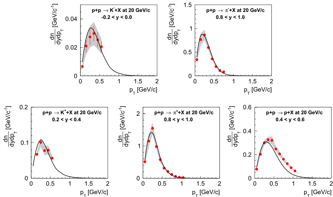
Fig. 23 Transverse momentum spectra of identified hadrons produced in inelastic p + p interactions at 20 GeV/c in selected rapidity intervals in comparison to the EPOS model [21] (black line). Systematic uncertainties are shown as shaded bands
