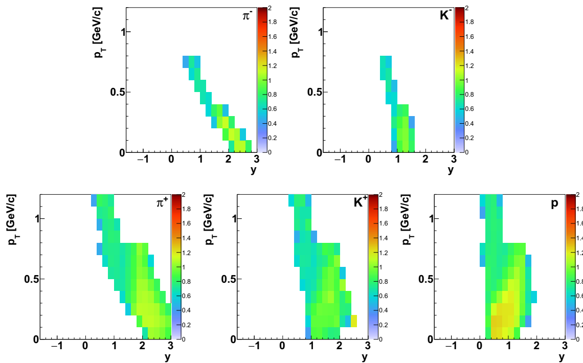
Fig. 12 Correction factors C_i^{-1} for the dE/dx identification method for positively and negatively charged pions, kaons and protons in p + p interactions at 20 GeV/c. The correction factor for antiprotons produced in inelastic p + p interactions is not presented due to insufficient statistics
