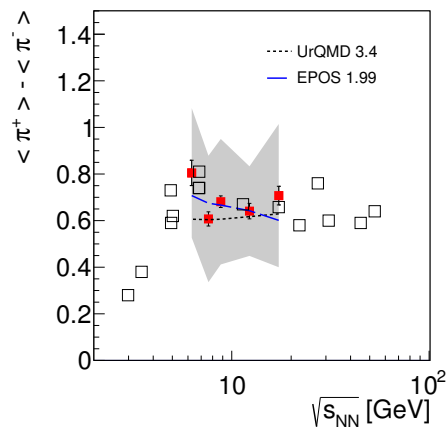
Figure 41: (Color online) Difference \langle \pi^+ \rangle - \langle \pi^- \rangle in inelastic p+p interactions as function of collision energy. Solid red squares depict NA61/SHINE results from this analysis, open squares show previously published measurements [11, 35, 36, 42]. Statistical uncertainties of the NA61/SHINE results are indicated by bars, systematic uncertainties by the shaded band. The EPOS [19] and UrQMD [25, 26] model predictions are shown as dashed and dotted lines, respectively.
