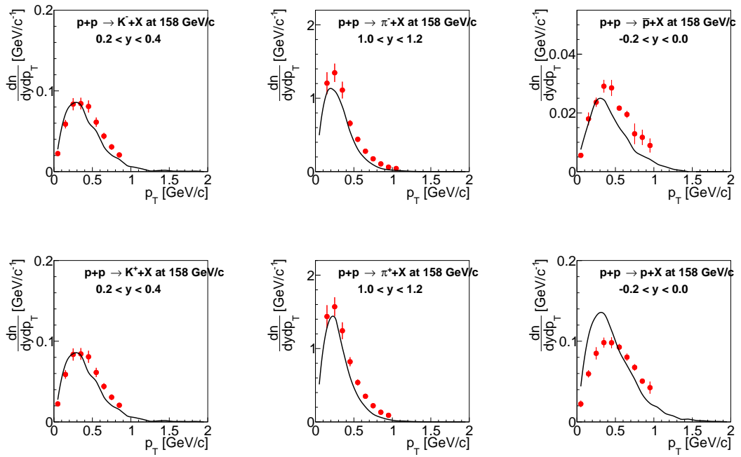
Figure 24: (Color online) Transverse momentum spectra of identified hadrons produced in inelastic p+p interactions at 158 GeV/c in selected rapidity intervals in comparison to the EPOS model [19] (black line). Only statistical uncertainties are shown for the data points. Systematic uncertainty of the presented results is at the level of 5-10%.
