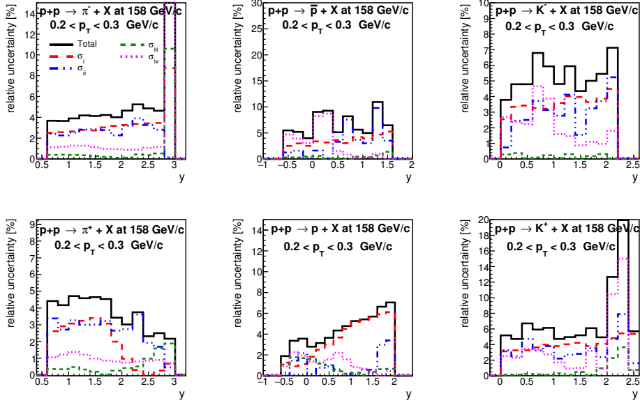
Figure 17: (Color online) Components of systematic uncertainty of particle spectra obtained from the dE/dx method in inelastic p+p interaction at 158 GeV/c as function of rapidity for the transverse momentum interval between 0.2 – 0.3 GeV/c. \sigma_i refers to removal of events with off-time beam tracks, \sigma_{ii} to possible bias of the S4 trigger, \sigma_{iii} to event and track selection procedure and \sigma_{iv} to the identification technique. Black lines (Total) show the total systematic uncertainty calculated as the square root of the sum of squares of the components.
