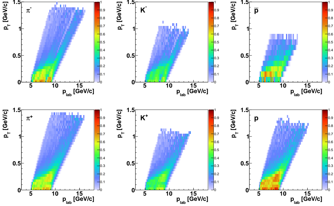
Figure 15: Efficiencies C_i^{tof} for the tof - dE/dx identification method for positively and negatively charged pions, kaons and protons for p+p interactions at 158 \text{ GeV}/c .
