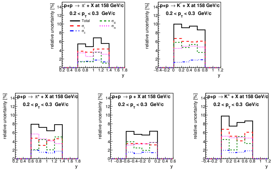
Figure 19: (Color online) Components of systematic uncertainty of particle spectra obtained from the tof - dE/dx method in inelastic p+p interaction at 158 GeV/c as function of rapidity for the transverse momentum interval between 0.2 – 0.3 GeV/c. \sigma_i refers to removal of events with off-time beam tracks, \sigma_{ii} to possible bias of the S4 trigger, \sigma_{iii} to event and track selection procedure and \sigma_{iv} to the identification technique. Black lines (Total) show the total systematic uncertainty calculated as the square root of the sum of squares of the components.
