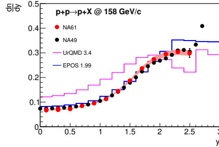
Figure 35: (Color online) Proton rapidity distribution in inelastic p+p interactions at 158 GeV/c compared with NA49 measurements [24] and predictions of the UrQMD [25, 26] and EPOS [19] models.
