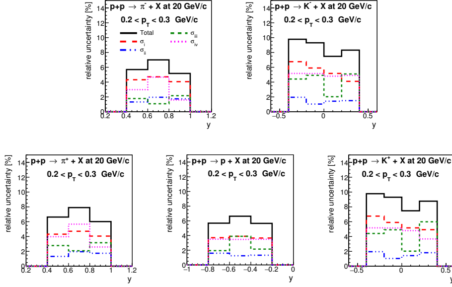
Figure 18: (Color online) Components of systematic uncertainty of particle spectra obtained from the tof-dE/dx method in inelastic p+p interaction at 20 GeV/c as function of rapidity for the transverse momentum interval between 0.2 – 0.3 GeV/c. \sigma_i refers to removal of events with off-time beam tracks, \sigma_{ii} to possible bias of the S4 trigger, \sigma_{iii} to event and track selection procedure and \sigma_{iv} to the identification technique. Black lines (Total) show the total systematic uncertainty calculated as the square root of the sum of squares of the components.
