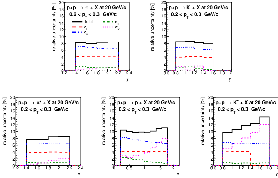
Figure 16: (Color online) Components of systematic uncertainty of particle spectra obtained from the dE/dx method in inelastic p+p interaction at 20 GeV/c as function of rapidity for the transverse momentum interval between 0.2 – 0.3 GeV/c. \sigma_i refers to removal of events with off-time beam tracks, \sigma_{ii} to possible bias of the S4 trigger, \sigma_{iii} to event and track selection procedure and \sigma_{iv} to the identification technique. Black lines (Total) show the total systematic uncertainty calculated as the square root of the sum of squares of the components.
