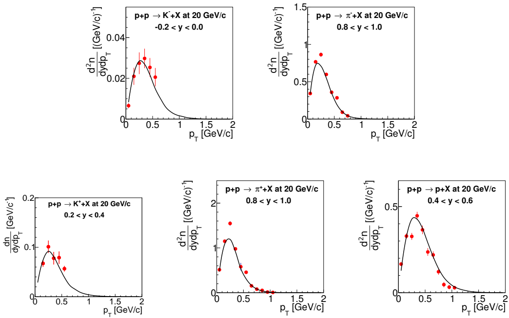
Figure 23: (Color online) Transverse momentum spectra of identified hadrons produced in inelastic p+p interactions at 20 GeV/c in selected rapidity intervals in comparison to the EPOS model [19] (black line). Only statistical uncertainties are shown for the data points.
