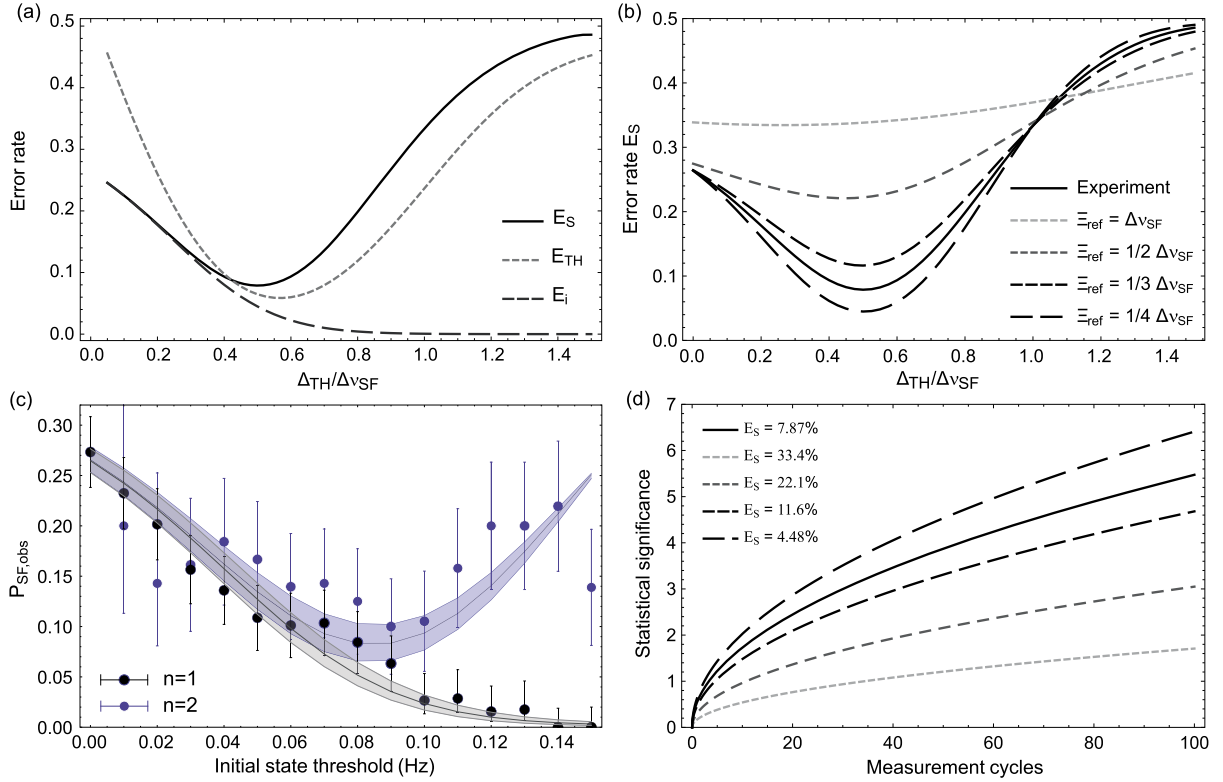
Fig. 5. (a) The scaling of the error rates as function of the threshold parameter \Delta_{TH} is shown for the threshold method error rate E_{TH} , for the initialization error rate E_i , and for the mean error rate of the spin-state assignment E_S . (b) The error rate E_S as function of \Delta_{TH} is shown for different ratios \Xi_{ref}/\Delta v_{SF} . (c) Observed spin-flip probabilities of simulated precision trap spin-flip drives with P_{SF,PT} = 0 . A simulated drive was inserted in the measurement sequence for each observed frequency shift with |\Delta_f| > 150 mHz. The observed spin-flip probability was evaluated with fixed threshold for the initial state, \Delta_i = 150 mHz, and varying the threshold parameter for the final state E_{f,n} for events requiring n = 1 (black data points) and n = 2 (blue data points) drives to identify the final state. The uncertainties of the data points originate from binomial or Poisson statistics. The results are compared to the theoretical expectations P_{SF,obs} = E_f(1 - E_{i,n}) + E_{i,n}(1 - E_f) shown as solid lines. The shaded area represent the uncertainty of the theoretical prediction due to the uncertainties of the parameters \Xi_{ref} , P_{SF} and \Delta v_{SF} . (d) The statistical significance s in standard deviations of distinguishing resonantly driven spin-flips of a saturated resonance in the PT from the background. The curve parameter is the error rate E_S . The parameters are corresponding to the minima of E_S of the curves shown in Fig. 5 (b). (For interpretation of the references to color in this figure legend, the reader is referred to the web version of this article.)
