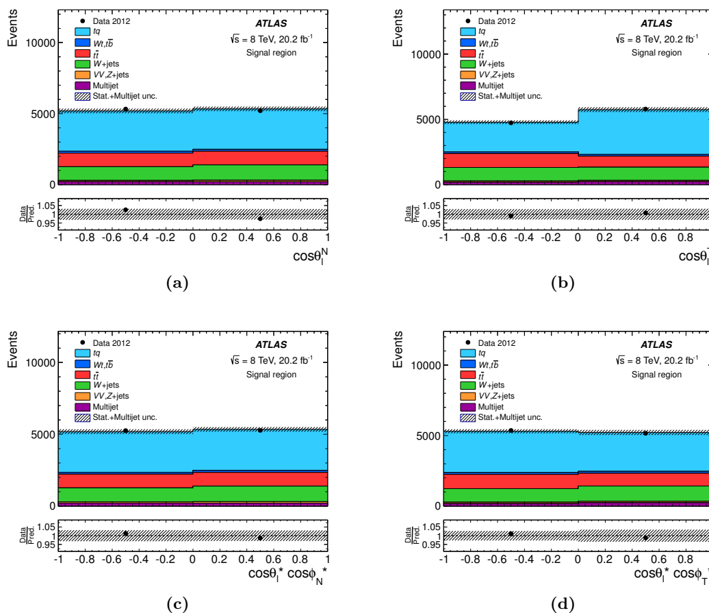
Figure 7. Distributions in the signal region of the angular observables used to measure the various asymmetries: (a) \cos \theta_{\ell}^N for A_{\text{FB}}^N , (b) \cos \theta_{\ell}^T for A_{\text{FB}}^T , (c) \cos \theta_{\ell}^* \cos \phi_N^* for A_{\text{FB}}^{N,\phi} , and (d) \cos \theta_{\ell}^* \cos \phi_T^* for A_{\text{FB}}^{T,\phi} . The observed distributions are compared to the predicted signal and background distributions, normalised to the results of the maximum-likelihood fit. The template t -channel distributions are taken from the baseline POWHEG-BOX sample. The labels tq and t\bar{b} refer to the t -channel and s -channel single-top-quark processes, respectively, and VV to diboson production. The uncertainty bands include the statistical post-fit uncertainty, the uncertainty due to the limited size of the simulation samples and the uncertainty in the normalisation of the multijet background, added in quadrature. The lower panels show the ratio of data to prediction.
